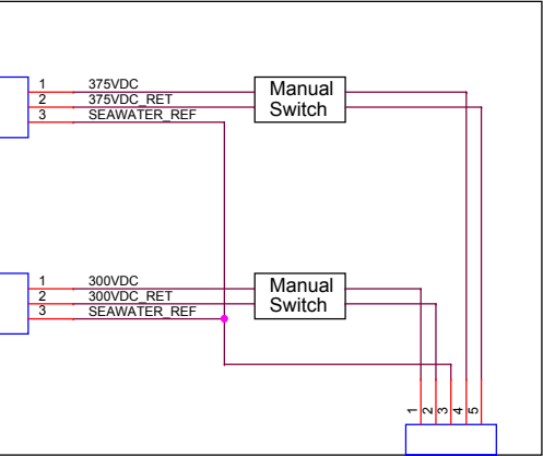
Diver Lockout Box
