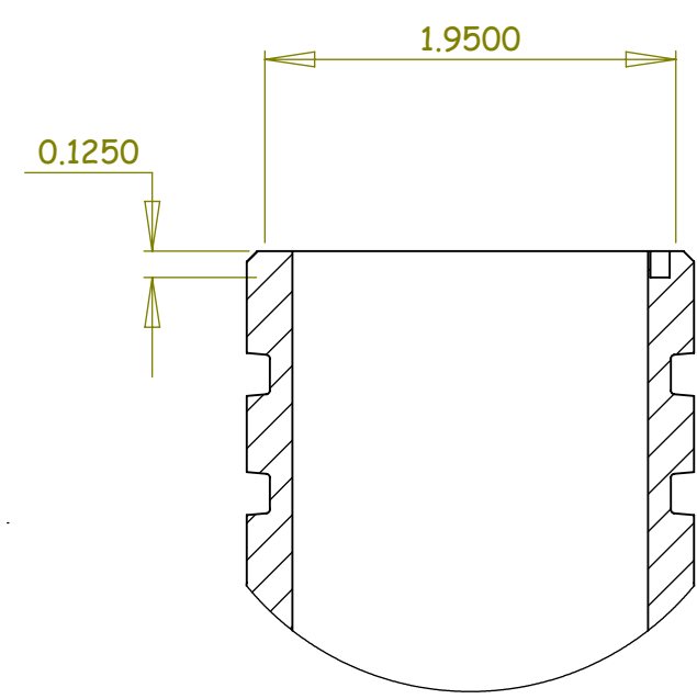
DETAIL D SCALE 1 : 1
