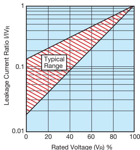
Leakage Current vs. Rated Voltage
