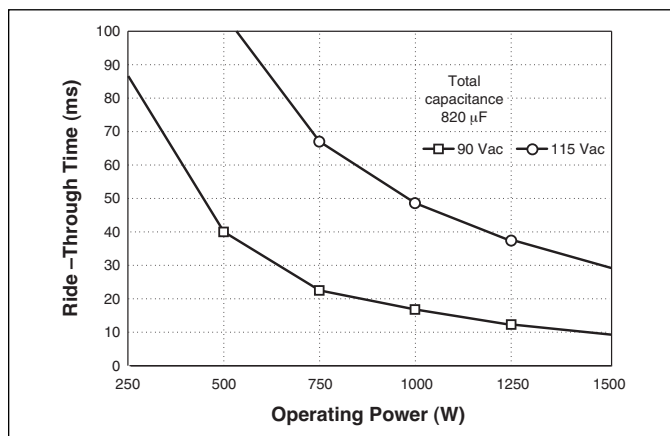
Figure 7-9 — Ride-through time vs. operating power
