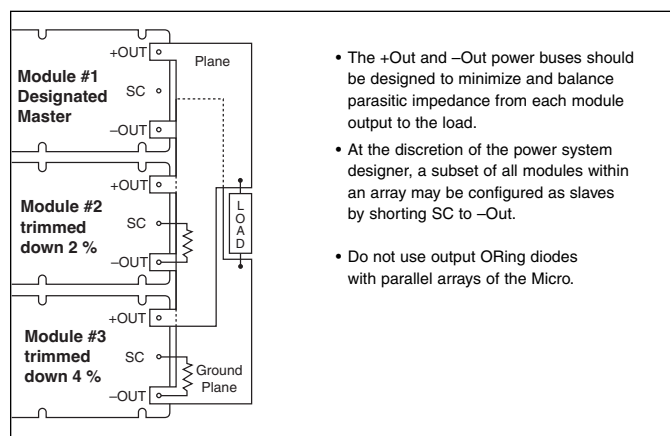
Figure 2–11 — Parallel module array output connections (Micro)
