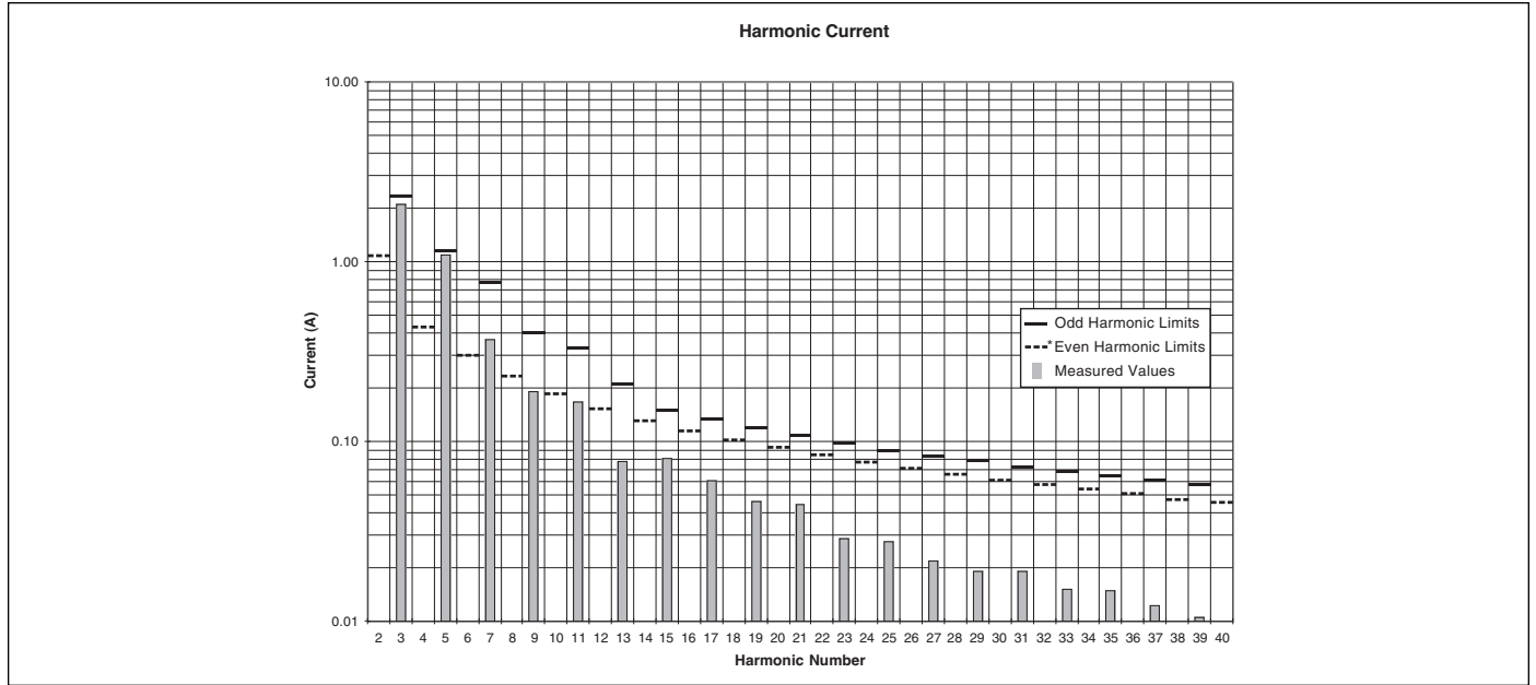
Figure 9-2 — Measured harmonic current at 230 Vac, 575 W vs. EN specs limits (*Measured values of even harmonics are below 0.01 A)
