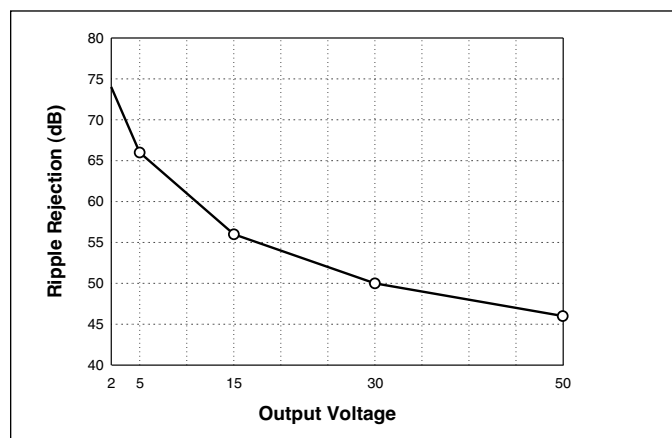
Figure 8-11 — Converter ripple rejection vs. output voltage (Typical)
