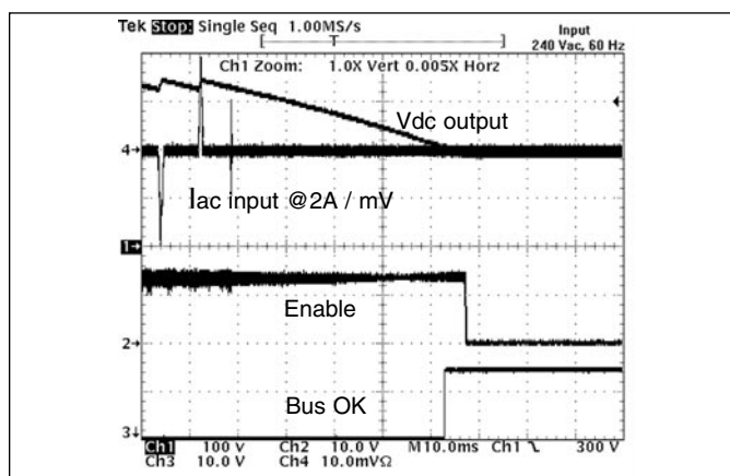
Figure 9-8 — Power down from 240 Vac
