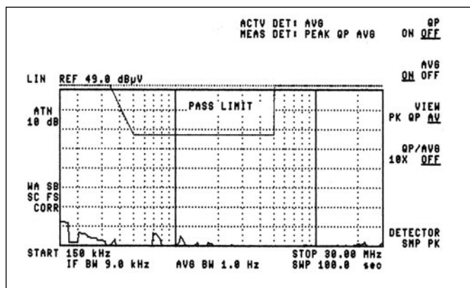
Figure 9-10c — Average detection
