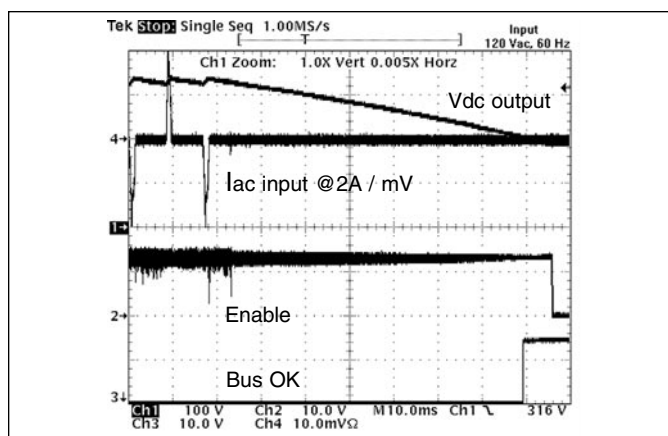
Figure 9-7 — Power down from 120 Vac
