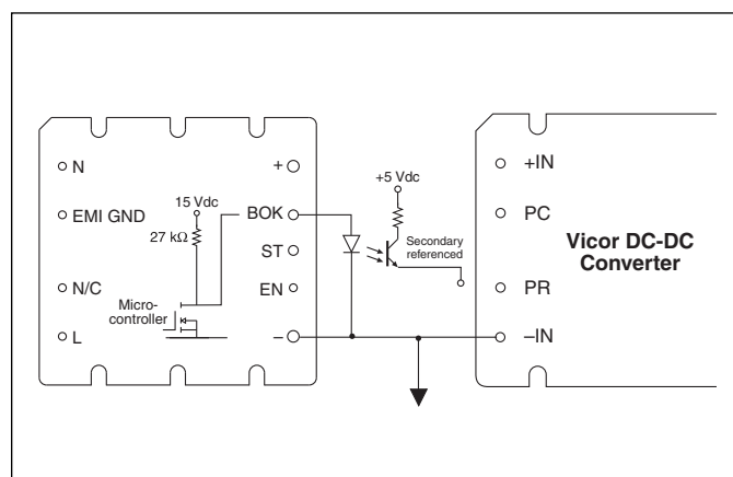
Figure 8–5 — Bus OK (BOK) isolated power status indicator
