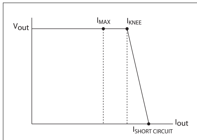
Figure 3-1 — Typical Maxi, Mini, Micro current limiting
