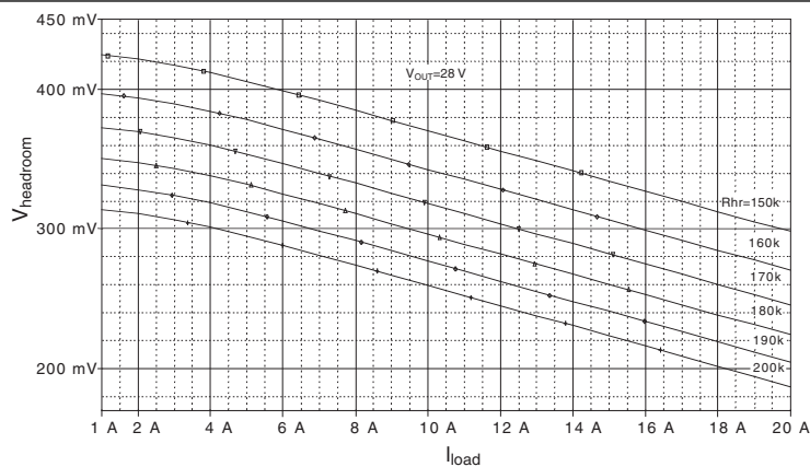
Figure 12-7 — Headroom vs. load current at 28 V output
