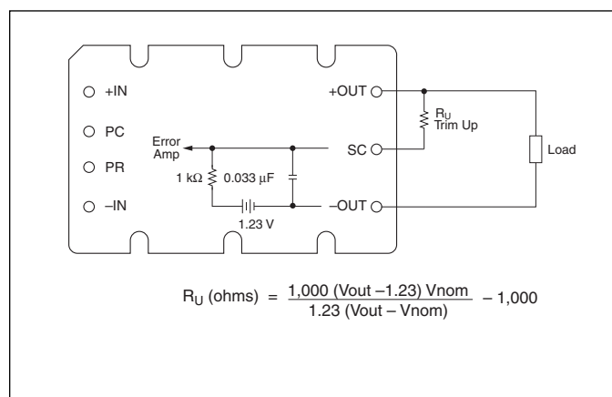
Figure 2-13b — Output voltage trim up circuit (Micro)
