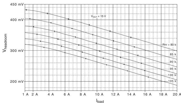
Figure 12-6 — Headroom vs. load current at 15 V output
