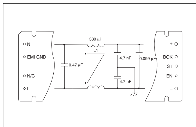
Figure 8–6 — Internal filter
