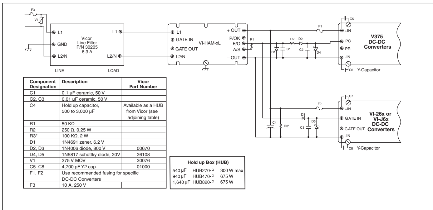
Figure 10-4 — Connection diagram HAM / DC-DC converter
