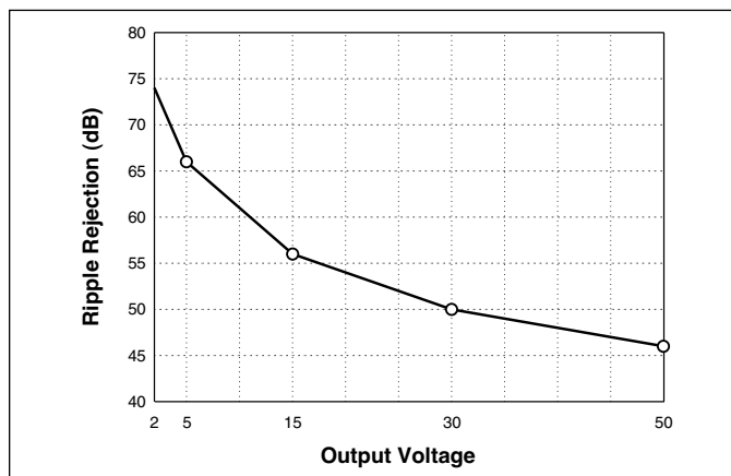
Figure 7-11 — Converter ripple rejection vs. output voltage (Typical)
