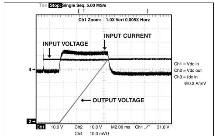
Figure 11-6 — Inrush limiting: Inrush current with 330 \mu F external capacitance Typical
