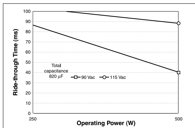
Figure 9-15 — Ride-through time vs. operating power
