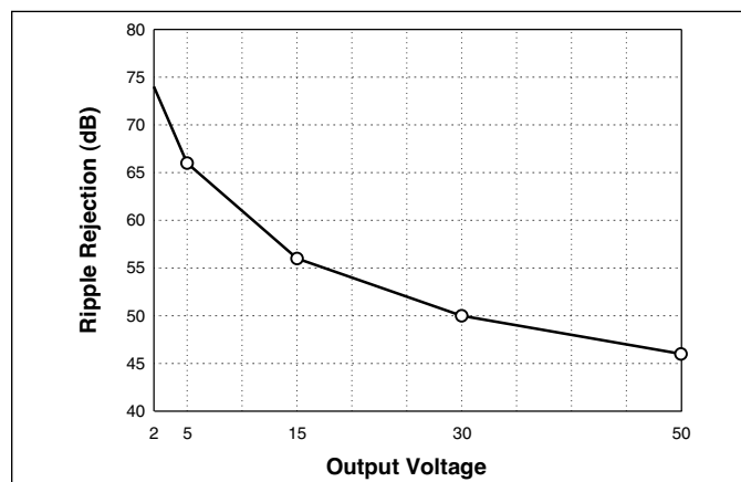
Figure 9-17 — Converter ripple rejection vs. output voltage (Typical)
