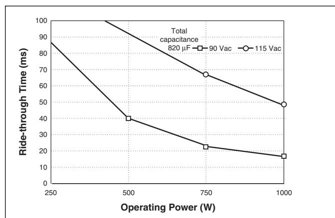
Figure 8-9 — Ride-through time vs. operating power
