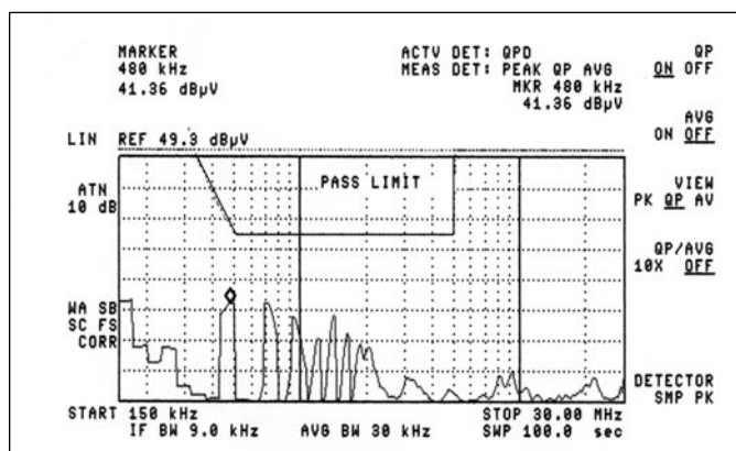
Figure 9-10b — Quasi-peak detection
