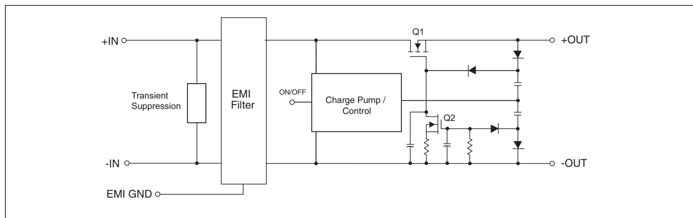
Figure 11-2 — Block diagram (FIAM)
