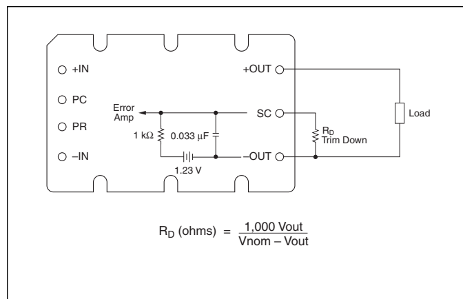
Figure 2-12b — Output voltage trim down circuit (Micro)
