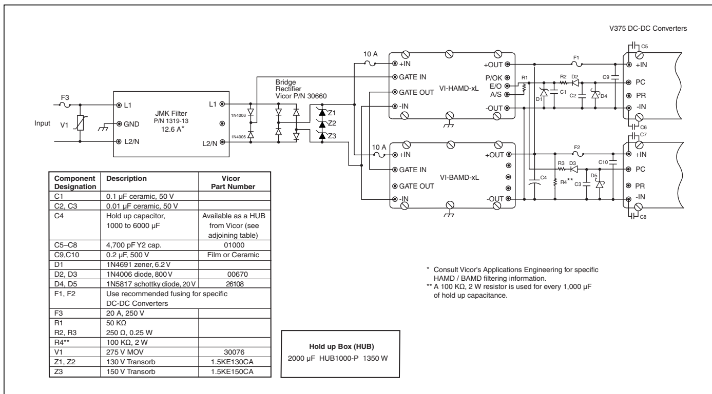
Figure 10-5 — Connection diagram, HAMD / BAMD / V375 DC-DC converters
