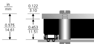
Figure 15-3 — Slotted baseplate; Height above board with standoff
