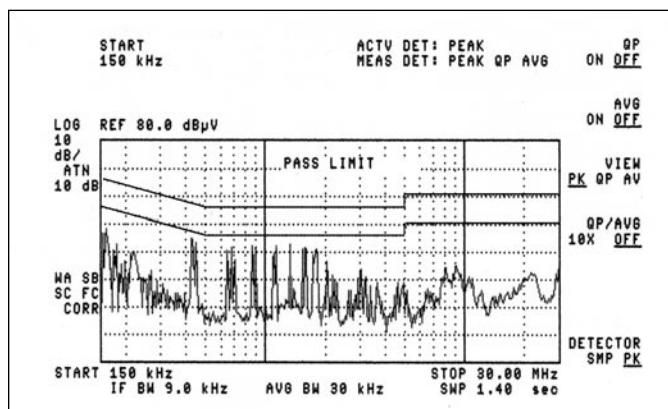
Figure 9-10a — Peak detection
