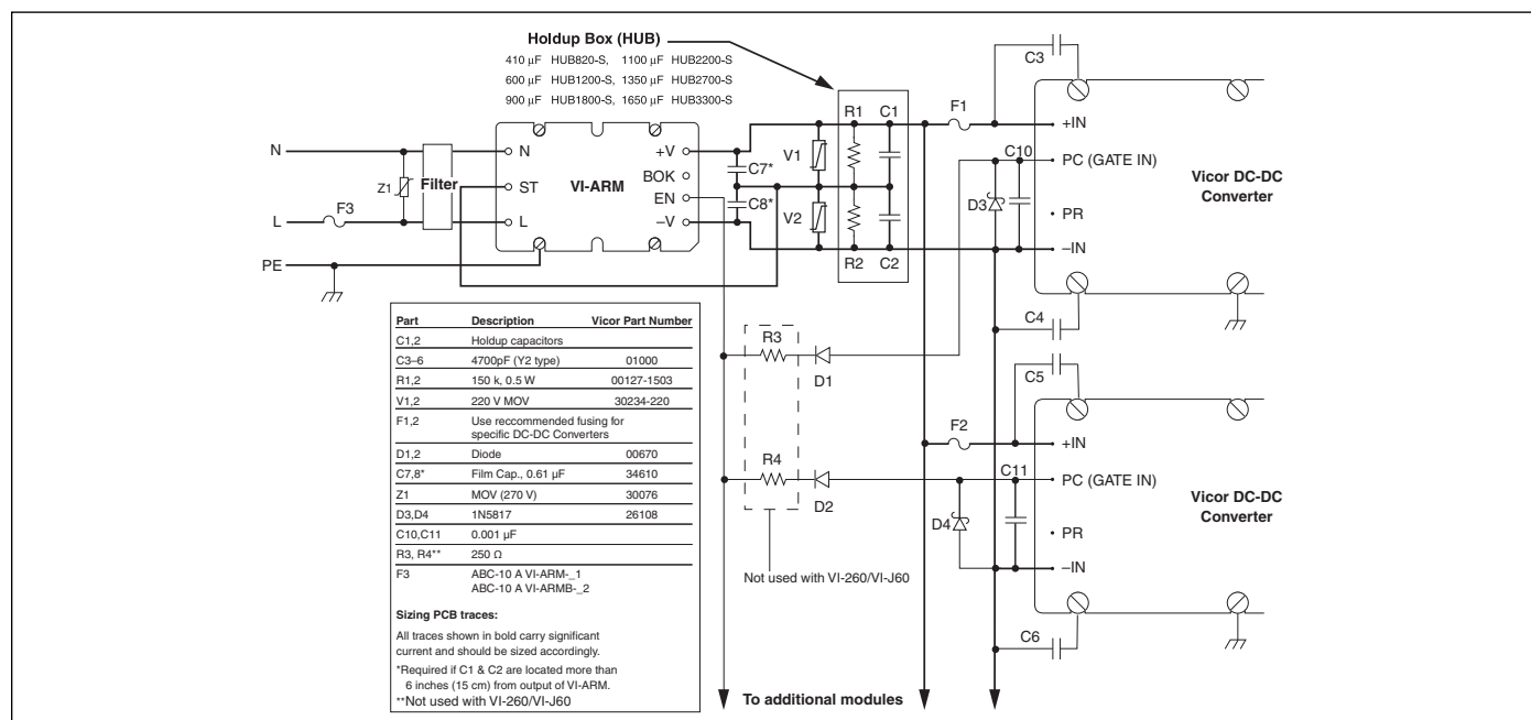
Figure 7–3 — Typical ARM application
