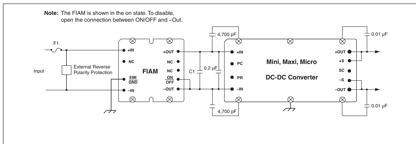
Figure 11-1 — Typical application (FIAM)
