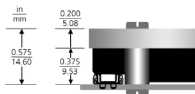
Figure 15-4 — Through-hole or threaded baseplate; Height above board with standoff
