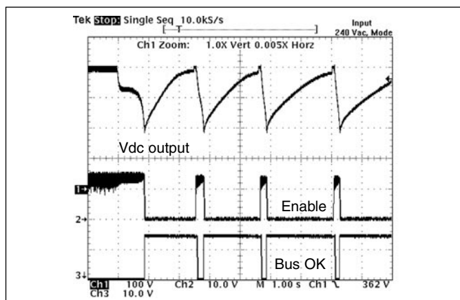
Figure 9-9 — Output overvoltage protection 240 Vac range
