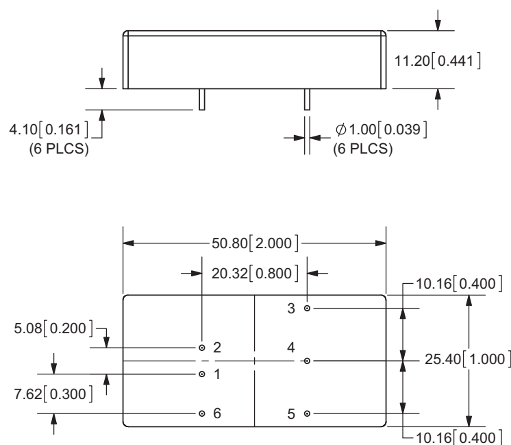
BOTTOM VIEW
