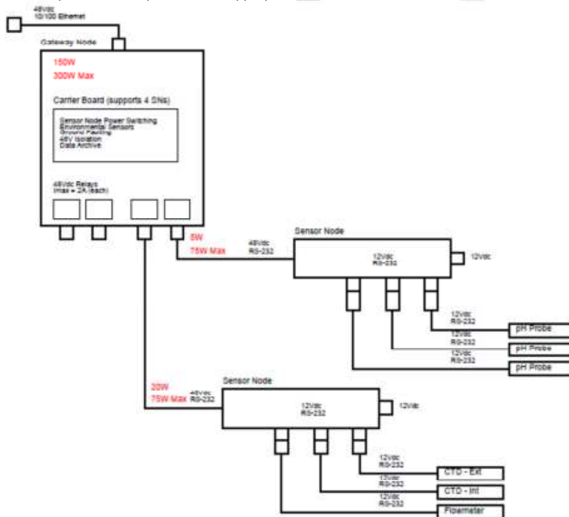
Figure 1: Possible Sensor Node configuration on swFOCE
