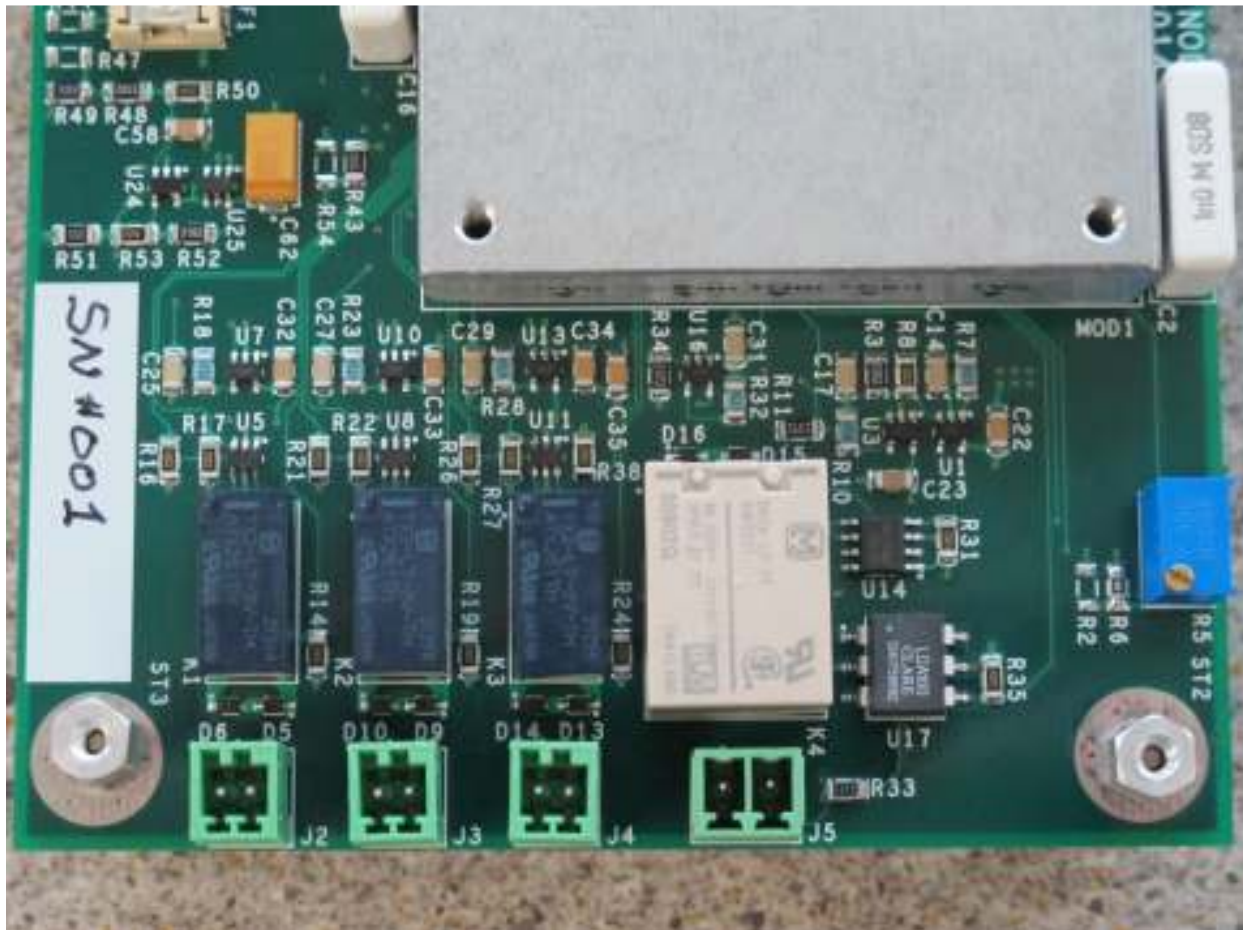
Figure 6: Output relays and connectors with trim circuit on far left (configured for trim up)
