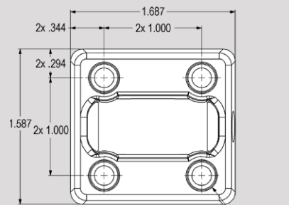
Mount Drawing
