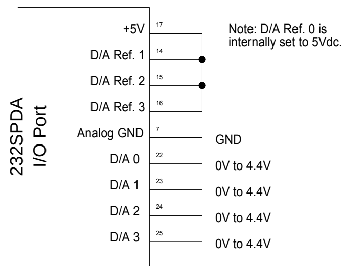
Figure 2.2 - Typical D/A Connections
