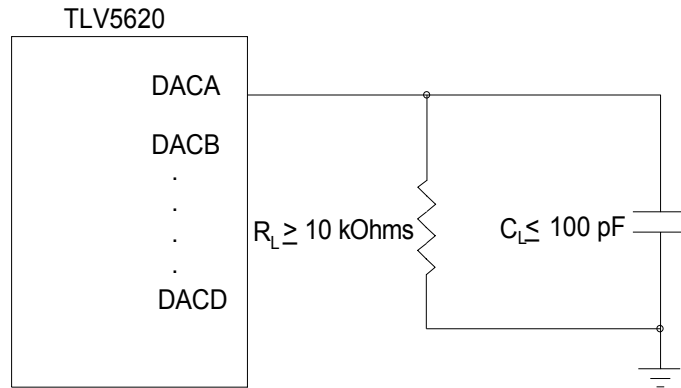
Figure D-1. Maximum D/A Load
