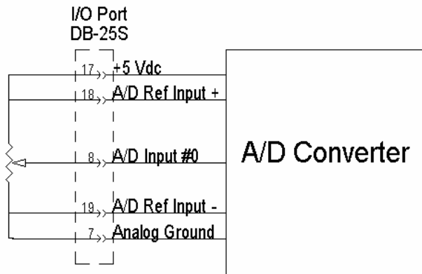
Figure 1.3 - A/D with Variable Resistor
