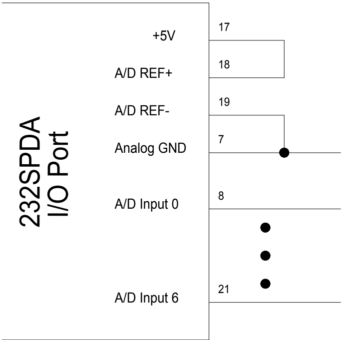
Figure 2.1 - Typical 0-5V A/D Connection
