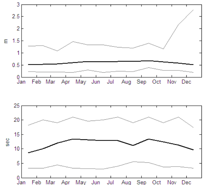
Figure 4. South shore Oahu wave climate 2004-2009:
