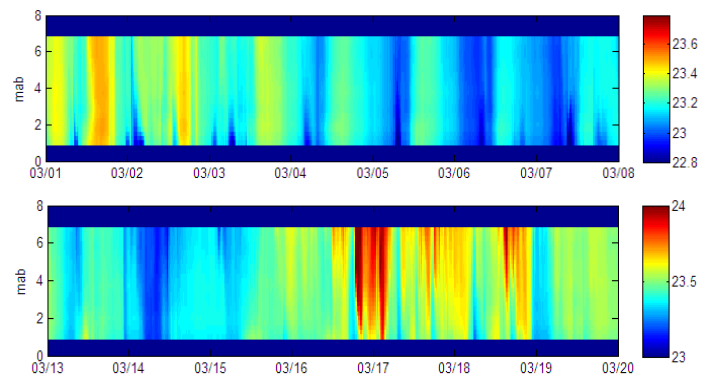
Figure 6. Temperature profiles from N12 thermistor chain for March 2009. Top panel illustrates diurnal cycle with intermittent cold intrusions near the bottom. Lower panel (one week later) shows occurrences of sudden warming events in the upper water column.
