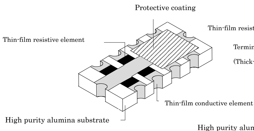
Fig.5 Chip resistor network (concave-type)
