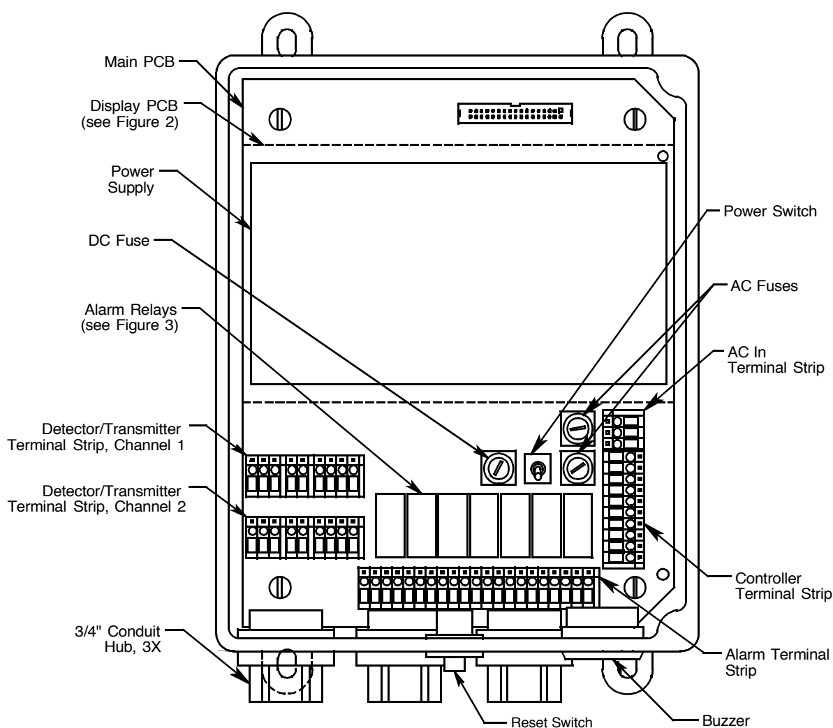
Figure 1. Beacon 200 Gas Monitor Component Location
