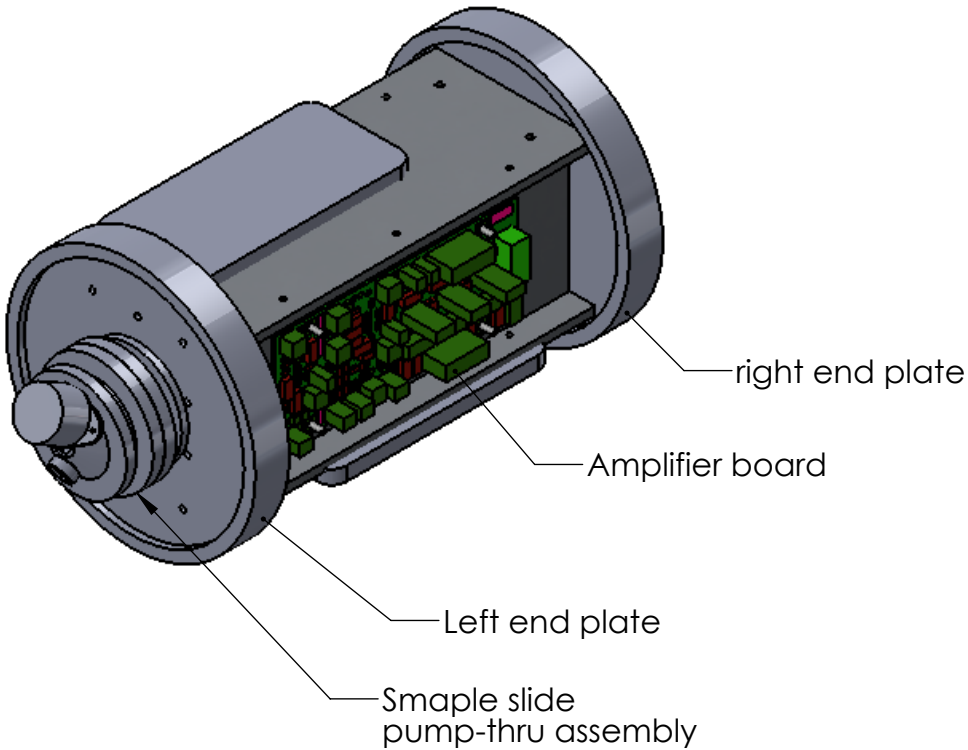
Electropack view (housing removed)
