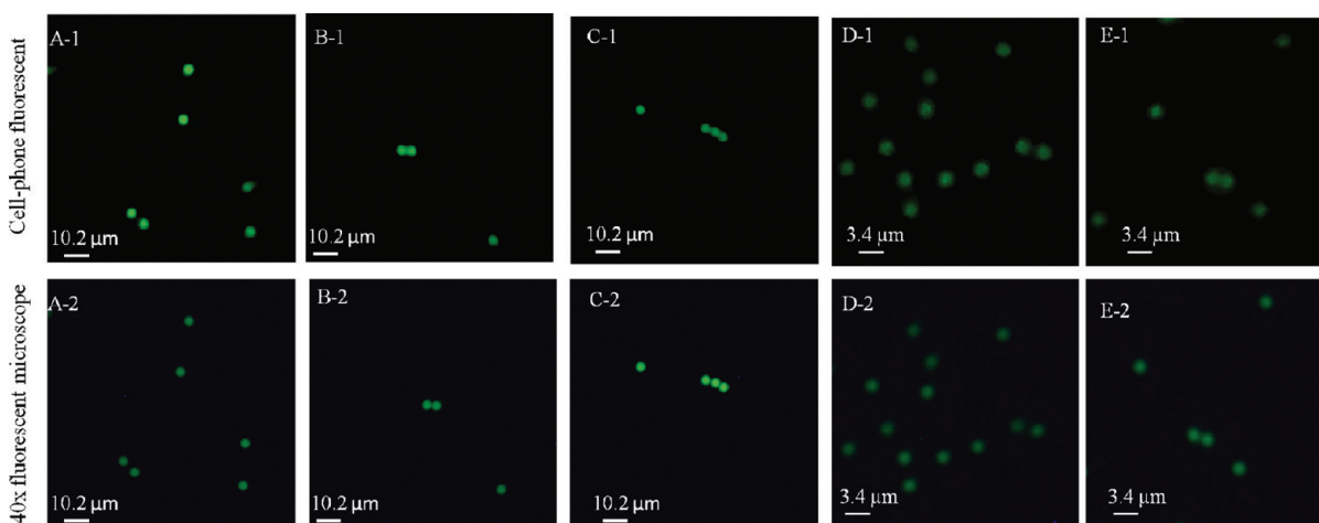
Figure 4. Spatial resolution of the optofluidic cell-phone fluorescent microscope shown in Figure 1 is quantified using green fluorescent beads with diameters of 4 and 2 \mu\text{m} . The top row shows the raw cell-phone images of these fluorescent beads, which demonstrate \sim 2 \mu\text{m} resolution; see, e.g., the touching 2 \mu\text{m} particles in panel E-1 that can be resolved. For comparison purposes, the bottom row shows the images of the same particles obtained using a 40\times microscope objective lens ( \text{NA} = 0.65 ) on a benchtop fluorescent microscope.
