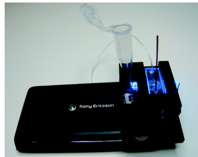
Cell-phone cytometer (Holomic LLC)
