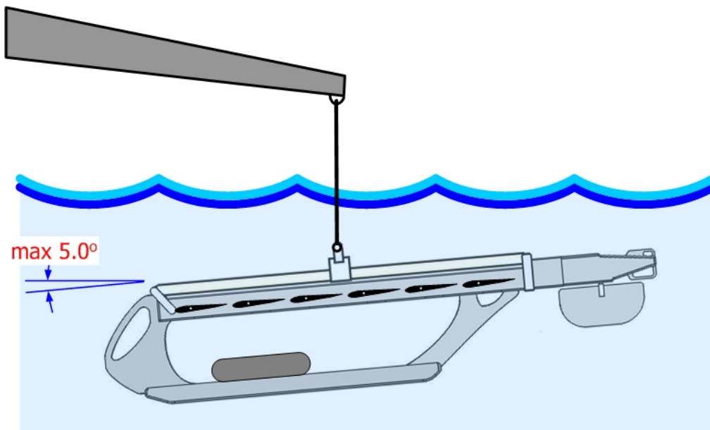
Figure 3-8: Checking Glider Underwater Balance
