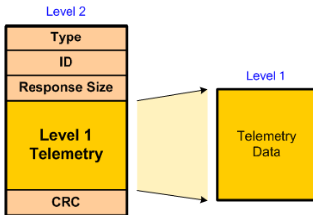
Figure 9-1: Level 2 Telemetry Data Packet
