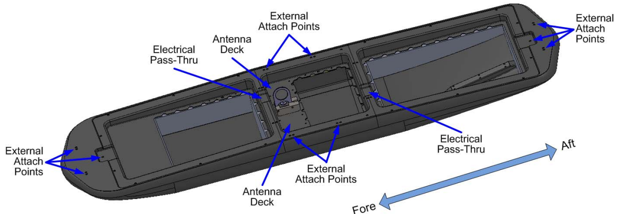
Figure 1-3: Basic Hull External Features
