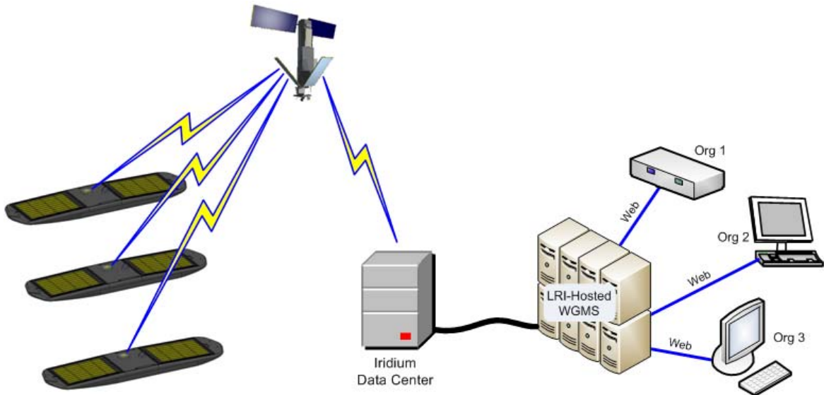
Figure 5-10: LRI-Hosted Shared WGMS
