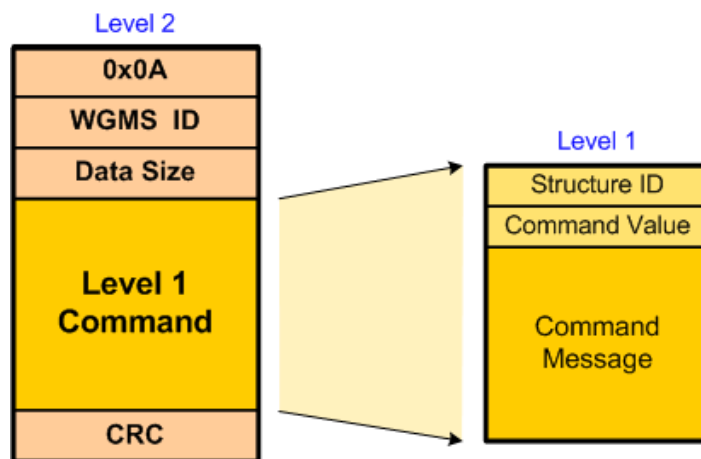
Figure 7-1: Command Packet Format
