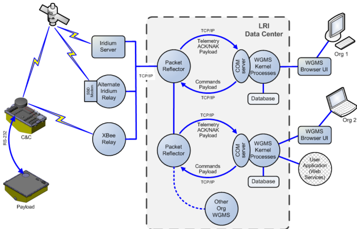
Figure 5-11: Multiple Orgs Using LRI-Hosted WGMS
