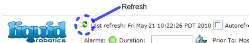
Figure 5-5: Refresh Icon
