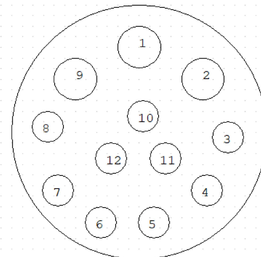
Wave Glider G-Port Male (Customer Supplied)
