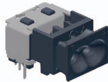
FIGURE 1 OptoLock connector.
