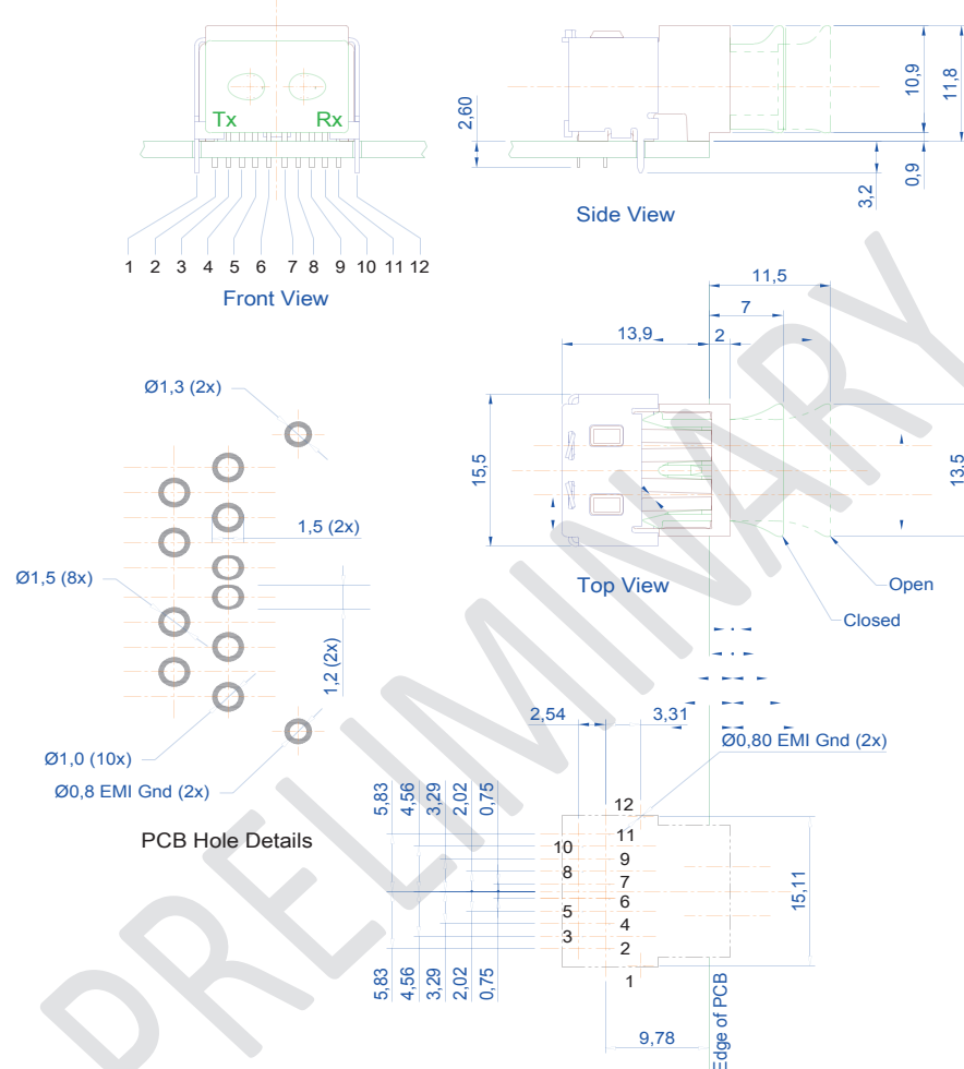
FIGURE 2 PCB layout footprint for IDL301T-220
