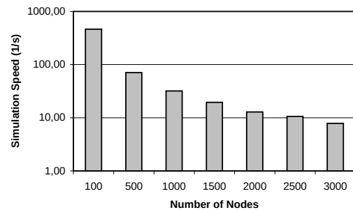
Fig. 5. Simulation speed with different number of nodes
