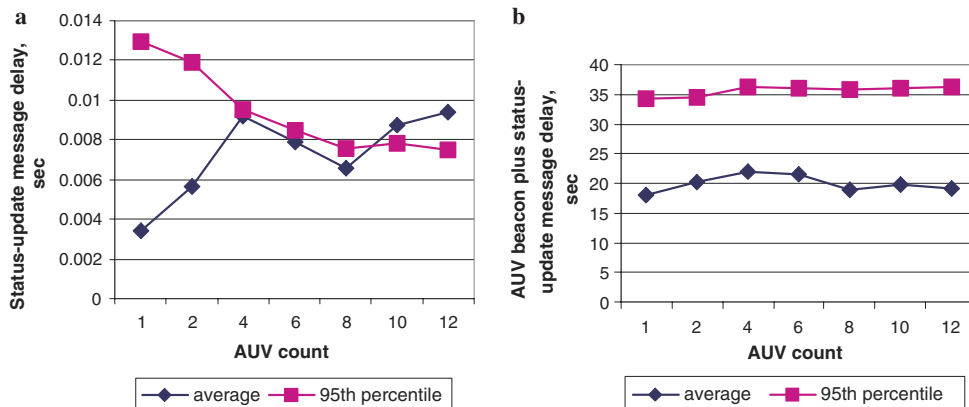
Fig. 5. Status-update message delays.
