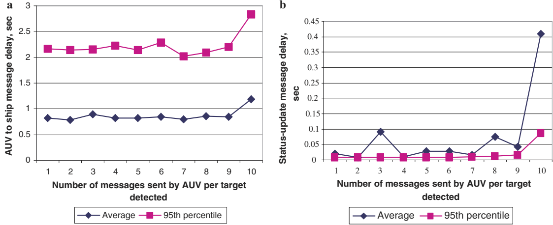
Fig. 10. AUV to ship and status-update message delay depending on the number of messages sent by AUV per target detected.
