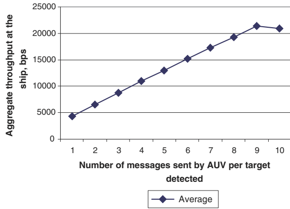
Fig. 11. Aggregate throughput at the ship depending on the number of messages sent by AUV per target detected.
