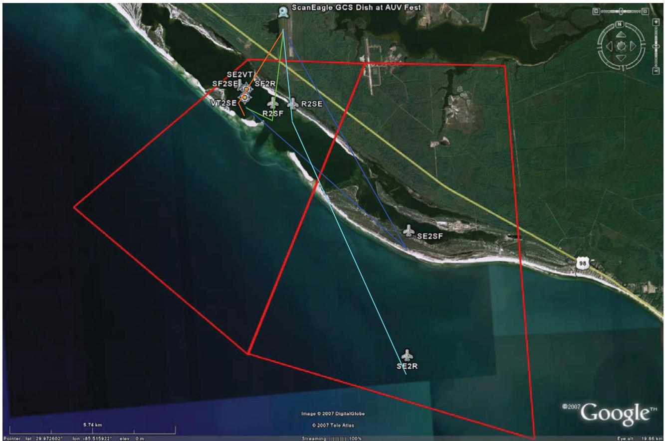
Figure 3 Minimum Separation for Autonomous Vehicles at AUV Fest 2007, Pindall AF
