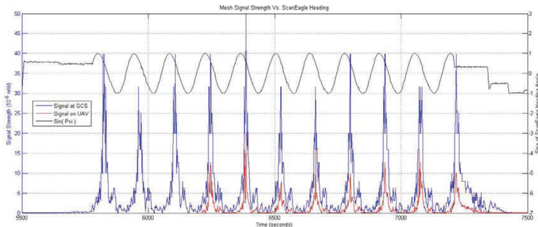
Figure 9 The data from Figure 8 plotted with a different zoom factor for clarity.
