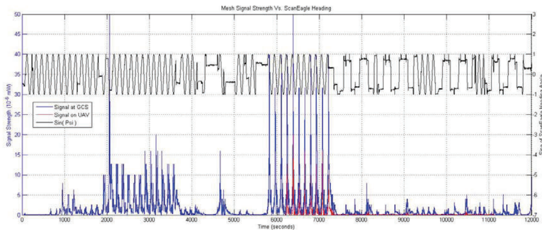
Figure 8 CS-to-UAV signal strength as measured by the CS and ScanEagle mesh cards plotted as a function of UAV heading to illustrate a strong correlation with aircraft attitude.
