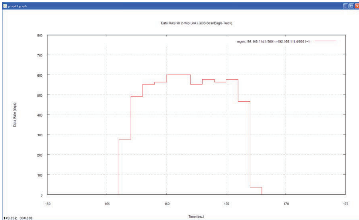
Figure 6 Received throughput of Mesh link from GCS to ScanEagle to ground vehicle
