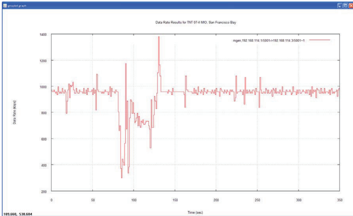
Figure 11 Received throughput of Mesh link from command ship to SeaFox
