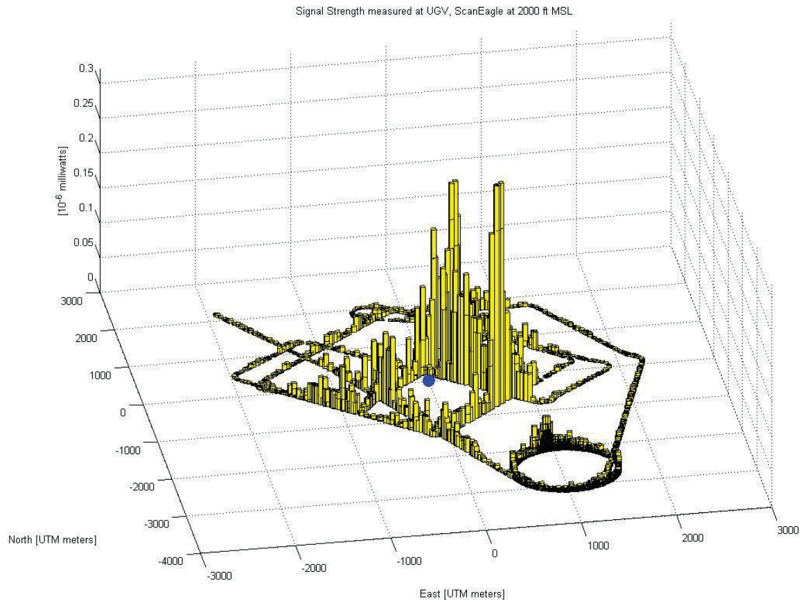
Figure 4 Mesh signal strength measured at UGV for ScanEagle at 2000 ft MSL
