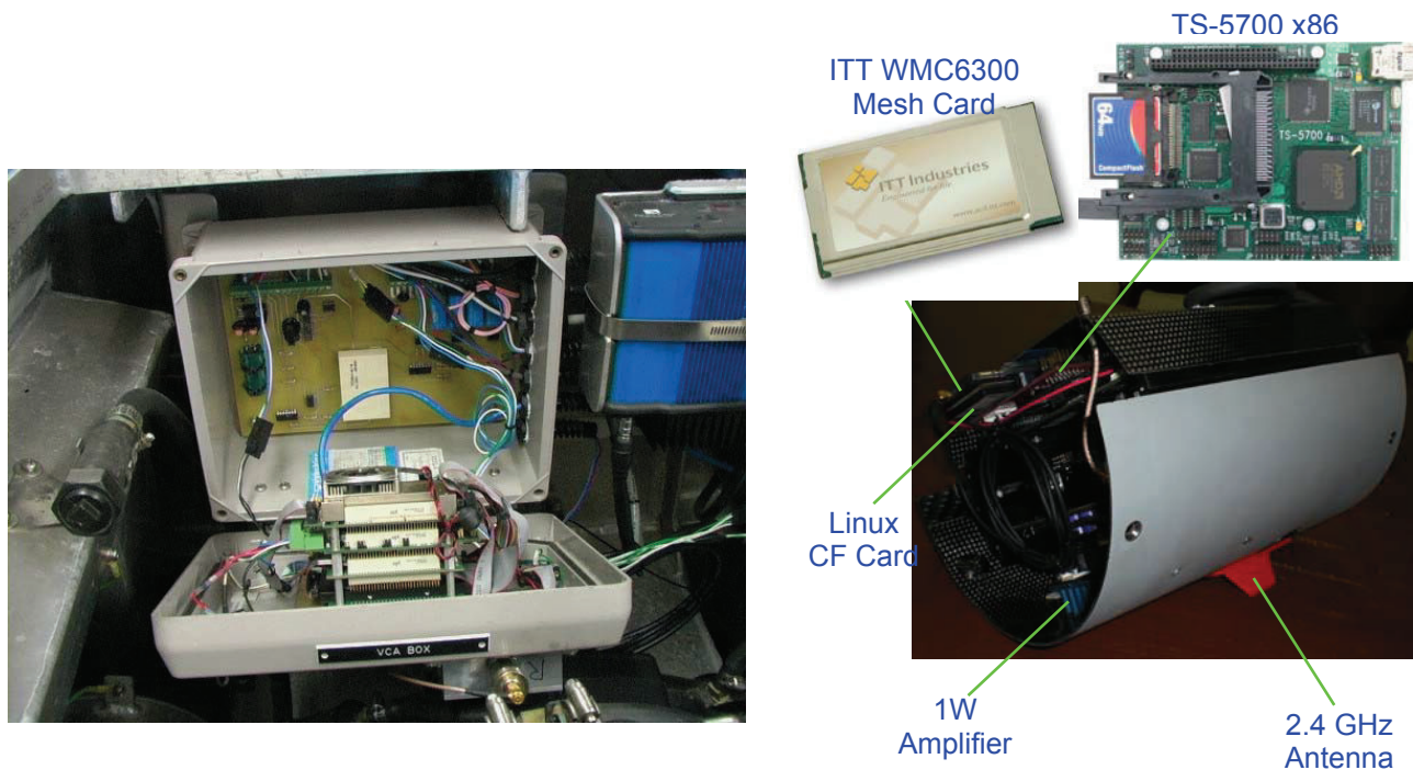
Figure 1 —SeaFox secondary computer (left) and ScanEagle avionics bay modifications (right).
