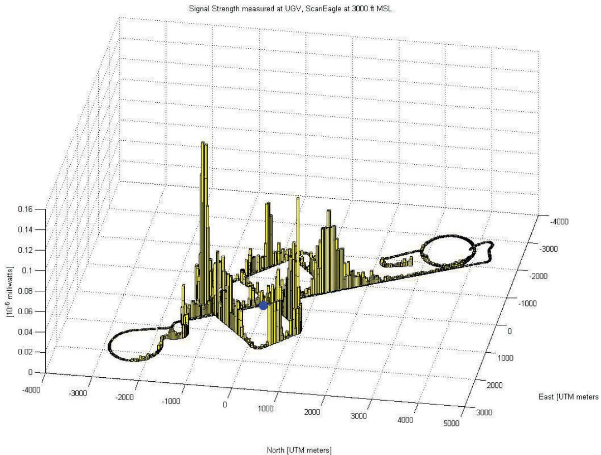
Figure 6 Mesh signal strength measured at UGV for ScanEagle at 3000 ft MSL
