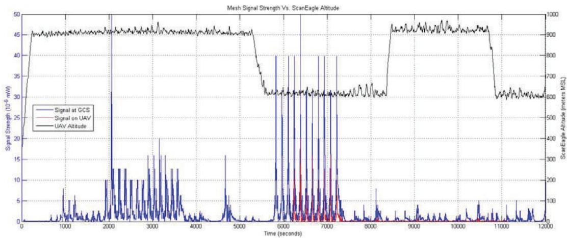
Figure 7 UAV altitude and GCS-to-UAV signal strength as measured by the GCS and ScanEagle Mesh cards
