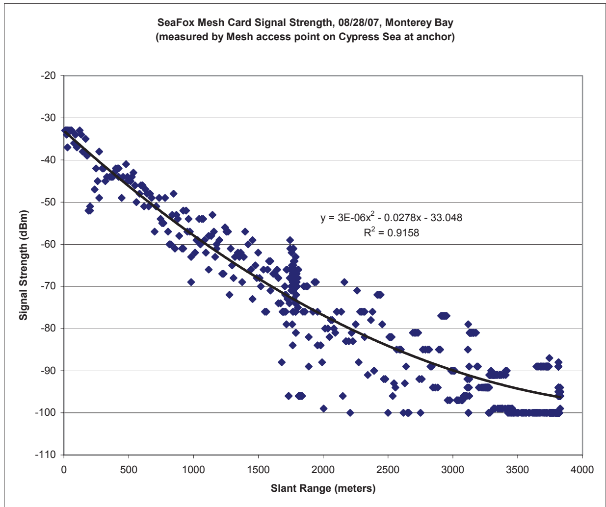
Figure 10 □ Command ship Mesh signal strength vs. separation distance as measured by SeaFo □
