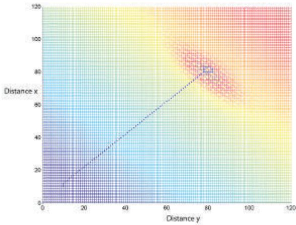
Figure 5. Simulated UAV Navigation using the APF Guidance Methodology
