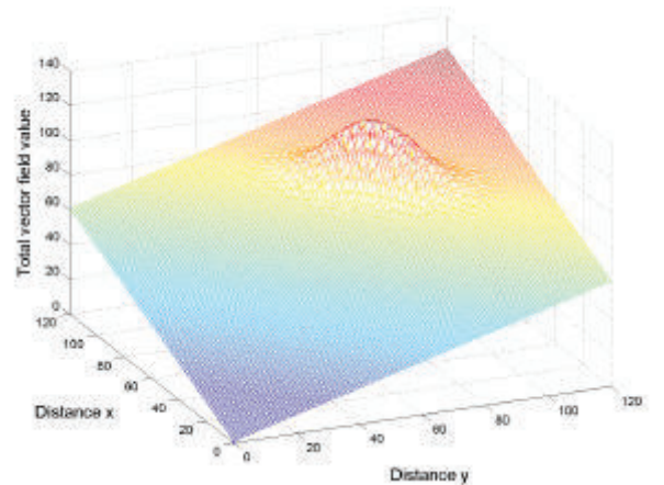
Figure 4. Example of a Total Vector Field
