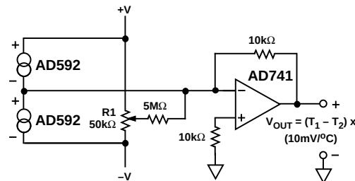
Figure 10. Differential Measurements
