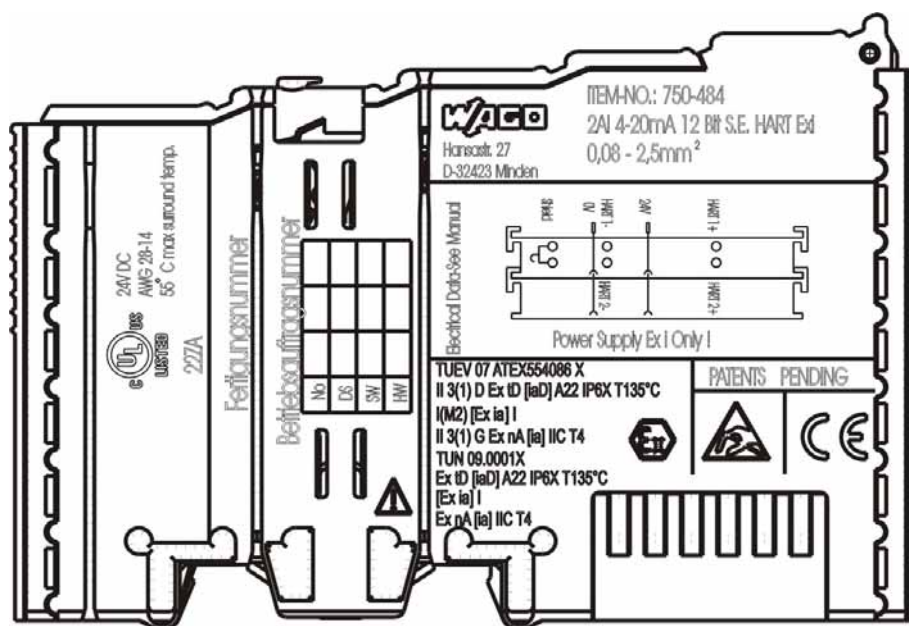
Figure 16: Side marking example for Ex i and IEC Ex i approved I/O modules according to CENELEC and IEC
