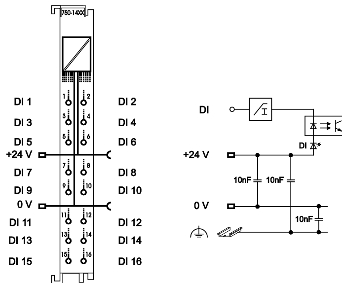
Figure 6: Schematic diagram
