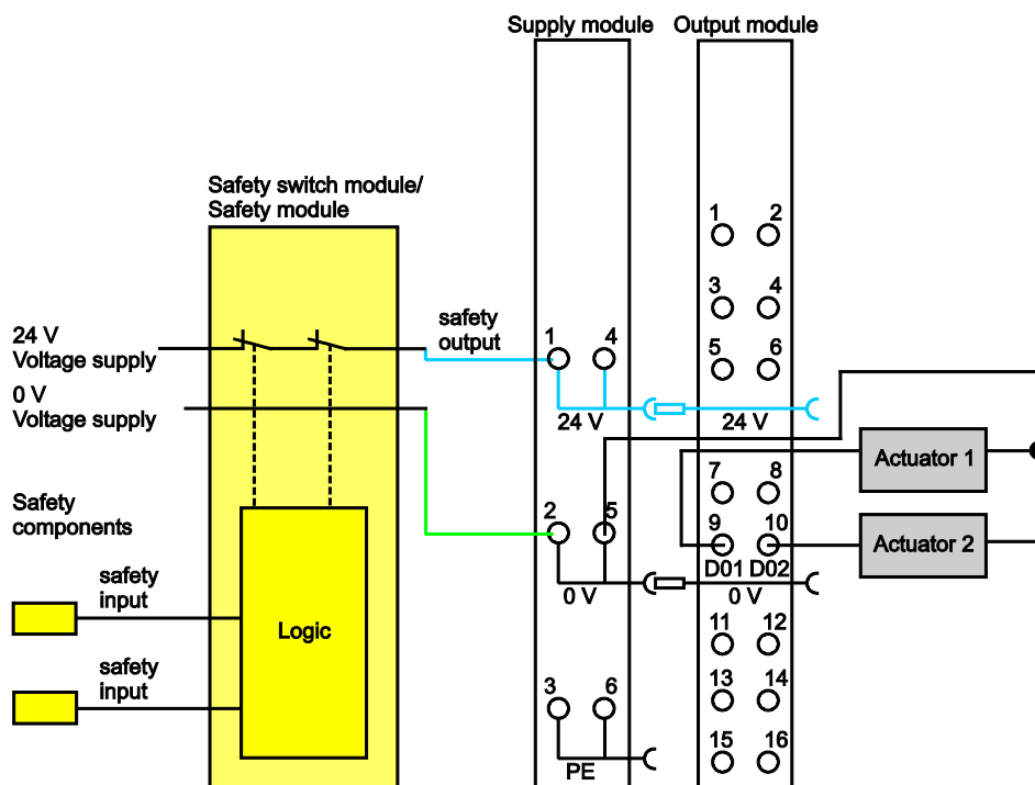
Figure 12: Two-channel single-pole disconnection
