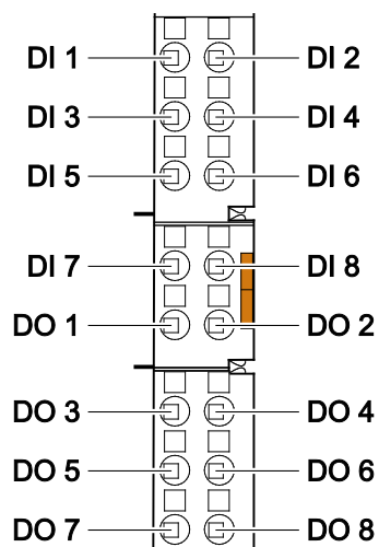
Figure 4: Connections
