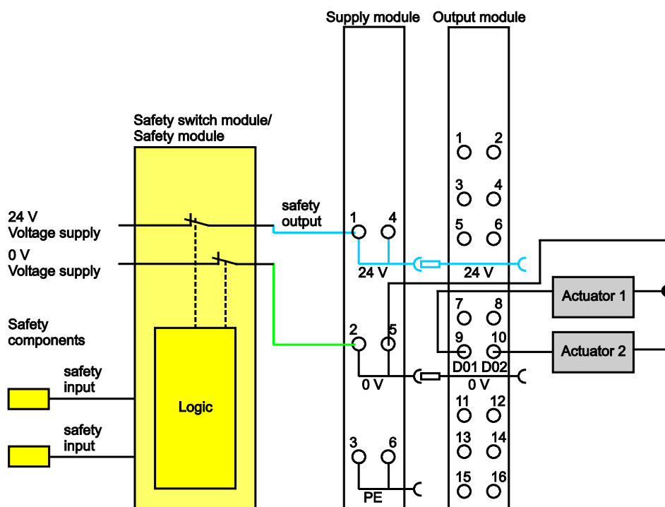
Figure 13: Two-channel double-pole disconnection
