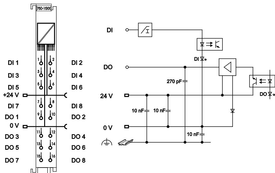
Figure 6: Schematic diagram
