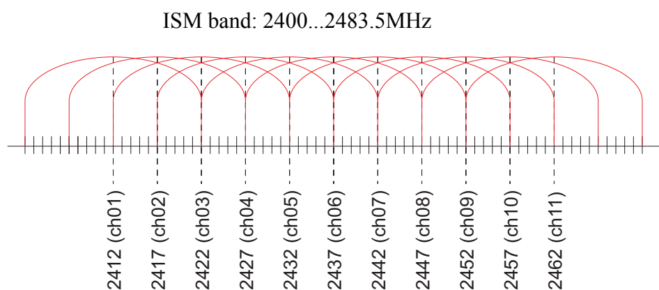
Figure 26: "Adaptive Frequency Hopping" (AFH) with WLAN example
