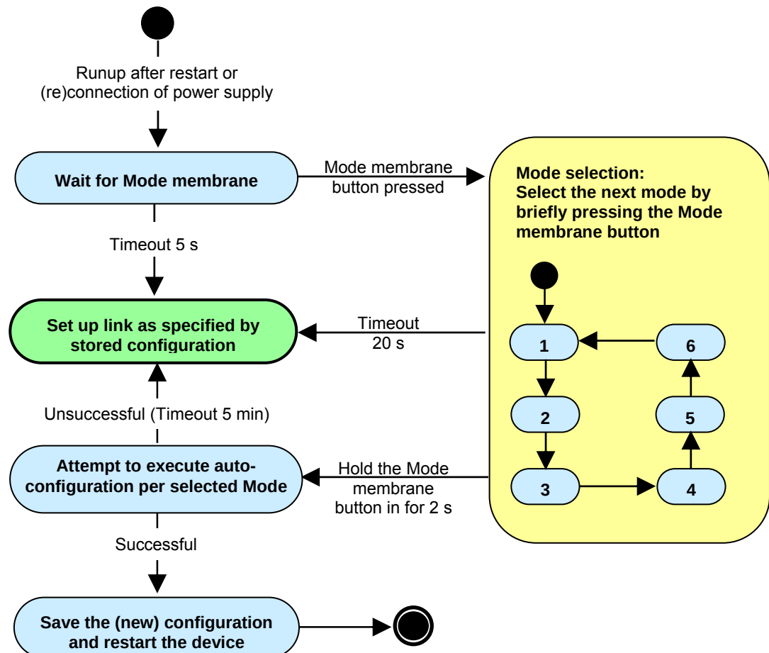
Figure 14: Flow chart
