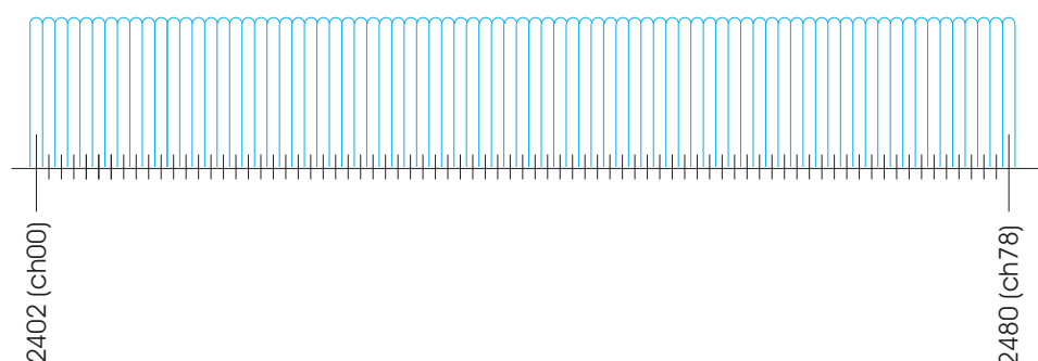
Figure 27: AFH with Bluetooth ® example
