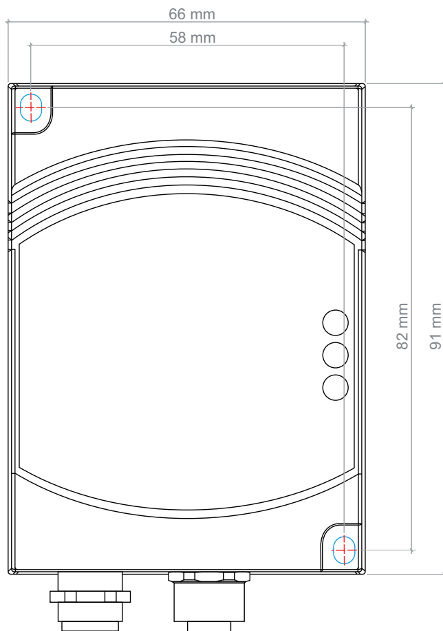
Figure 11: Drilled holes for attaching the BTEG
