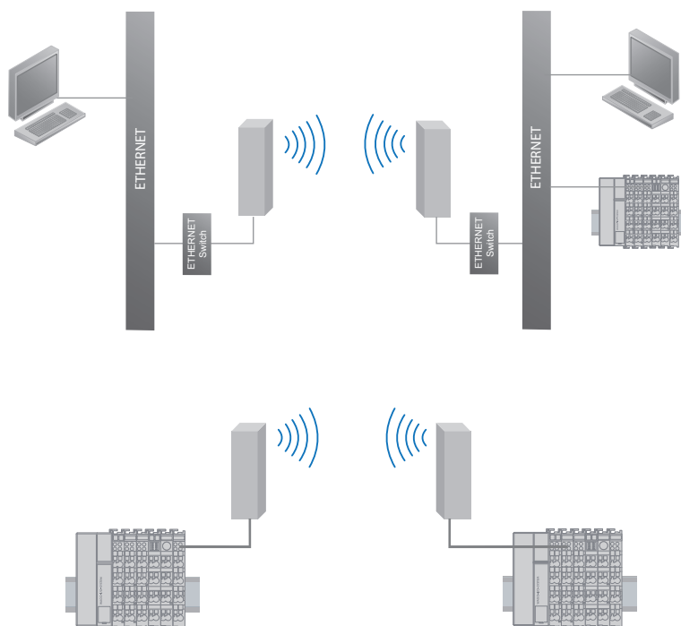
Figure 23: BTEG-BTEG bridge
