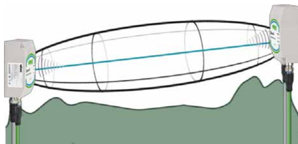
Figure 31: Fresnel zone
