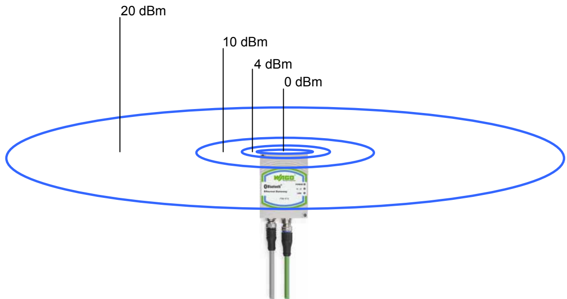
Figure 25: Range and limiting of transmitting power
