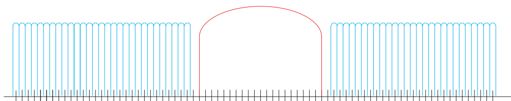
Figure 28: AFH with Bluetooth® and WLAN example
