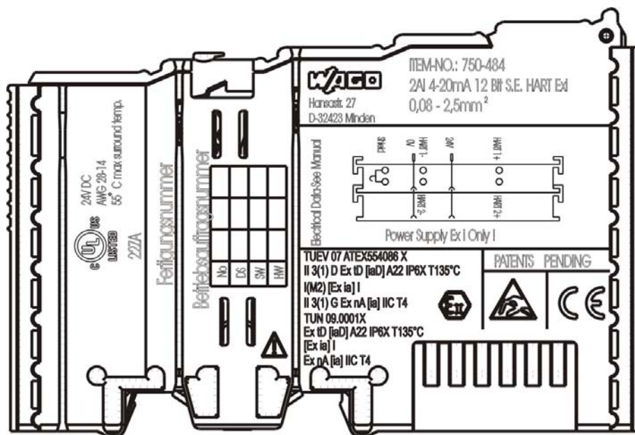
Figure 8: Example of side marking of Ex i and IEC Ex i approved I/O modules
