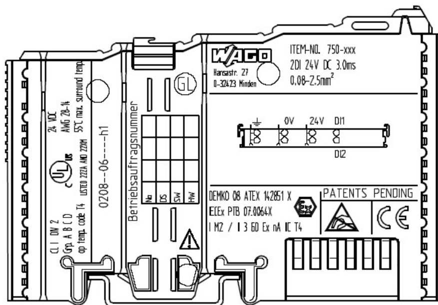
Figure 10: Example for lateral labeling of bus modules
