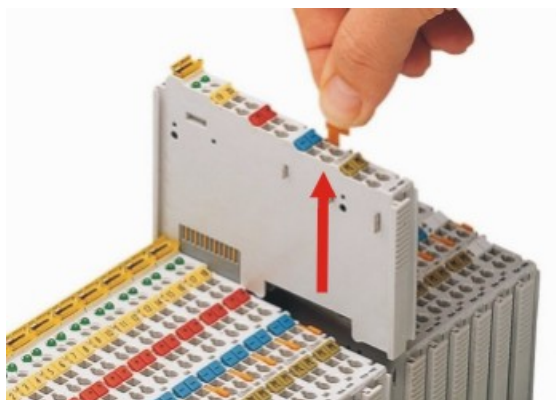
Figure 5: Removing the I/O module
