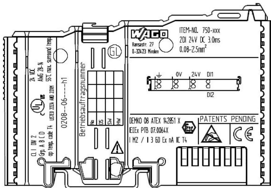
Figure 6: Example for lateral labeling of bus modules
