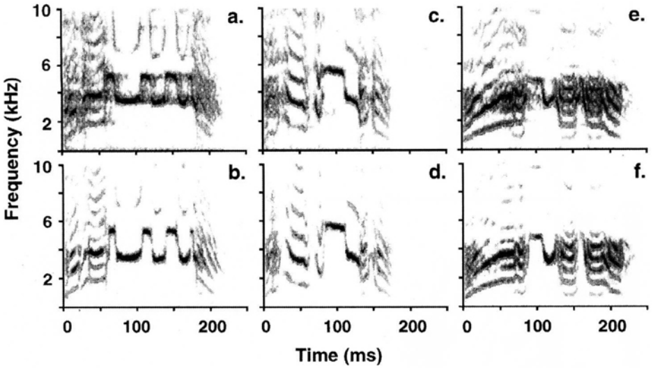
Figure 3. Spectrograms of actual Aratinga contact calls (3a,c,e) and their synthetic replicas (3b,d,f). The individuals and call types are Thalia (3a,b), Randy (3c,d), and Thoreau (3e,f).
