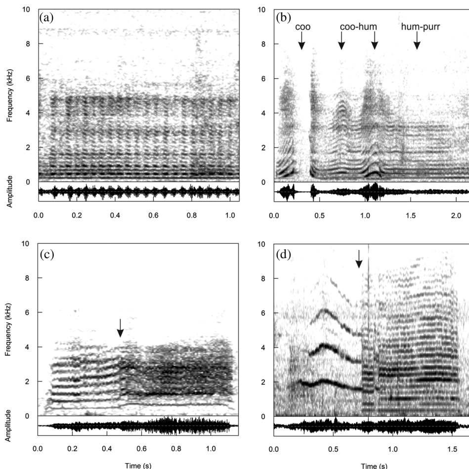
FIG. 5. Spectrograms and oscillograms (bottom) of vocalizations emitted by giant otters in the southern Pantanal of Brazil: (a) combination of hum and purr sounds (hum-purr, FFT = 1024 ), (b) gradation among affiliative sounds (coo, coo-hum, and hum-purr, FFT = 1024 ), (c) adult scream with a harsh, noisy ending (arrow indicates the transition, FFT = 512 ), (d) transition between cub high scream and cub scream (arrow indicates the transition, FFT = 1024 ).
