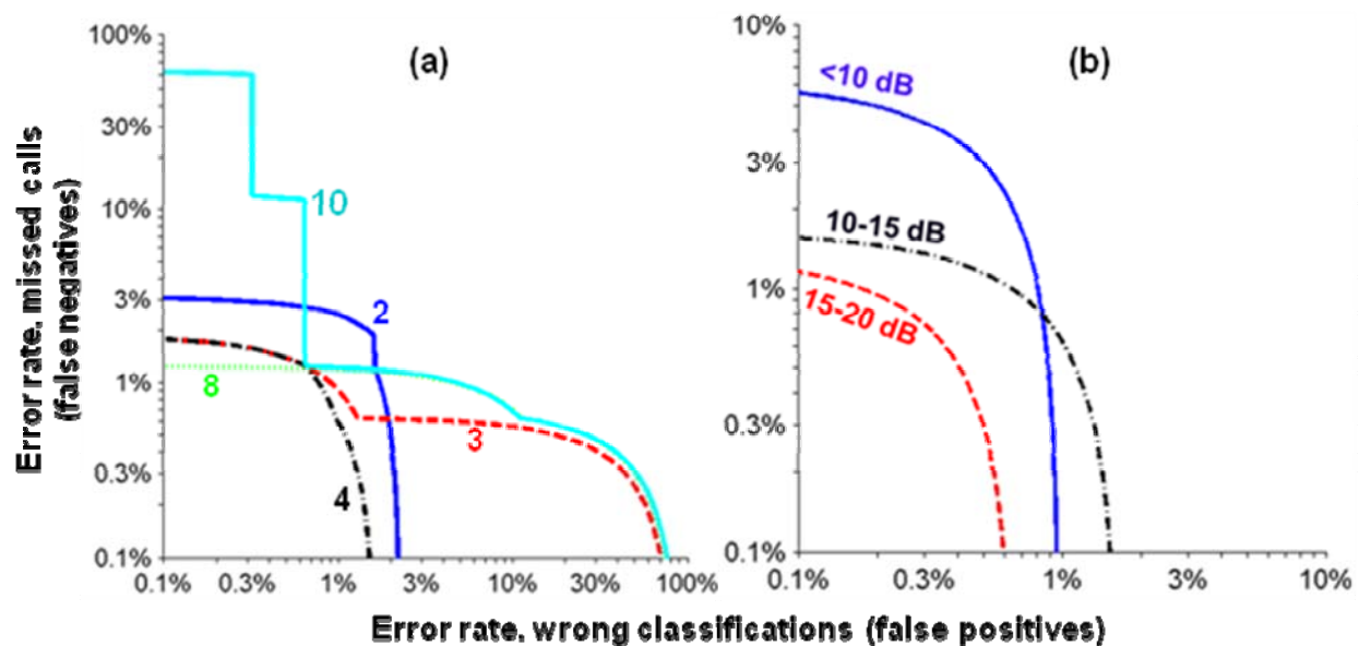
Fig. 2. Receiver Operating Characteristic curves for the neural network detector applied to the training data. Values near the lower left corner, representing smaller numbers of false detections and missed calls, are better. (a) ROC curve for different numbers of hidden units in the neural network. [The 8-hidden-unit curve is hidden by the 10-hidden-unit curve to the right of the 1% false positive point.] (b) ROC curves for the 4-hidden-unit network, with the curve for each 5-dB SNR bin plotted separately. The bin with SNR greater than 20 dB had no missed calls, and so could not be plotted on a logarithmic scale.
