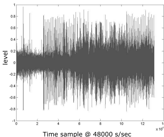
Fig. 4 Raw hydrophone signal
