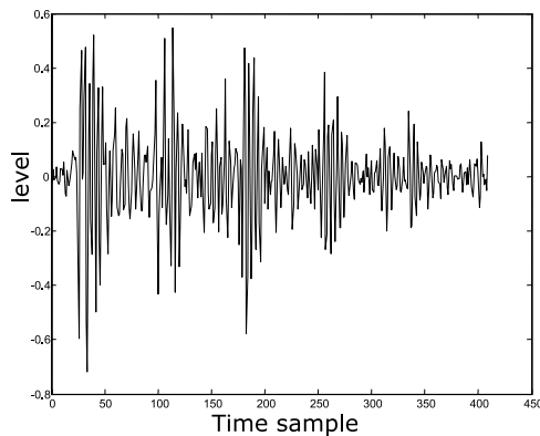
Fig. 12 Isolated click on left hydrophone
