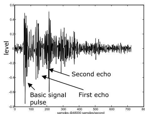
Fig. 9 Typical click showing multiple pulse structure
