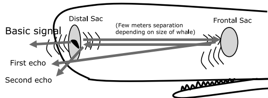
Fig. 8 Multiple pulse generation in the sperm whale
