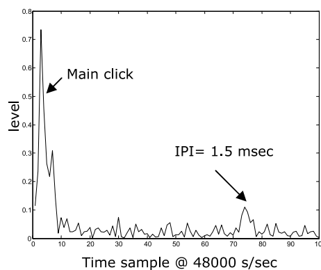
Fig. 11 Cepstrum of creak click B1
