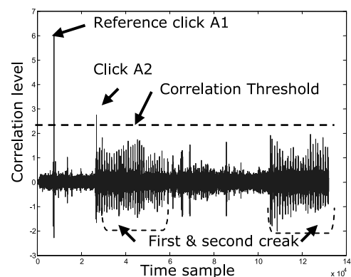
Fig. 6 Correlation with click A1
