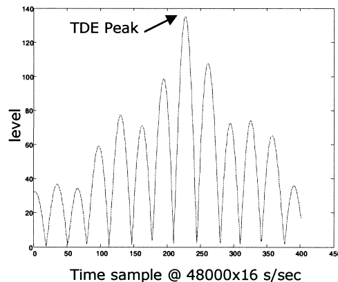
Fig. 15 Expanded view of the cross-correlation
