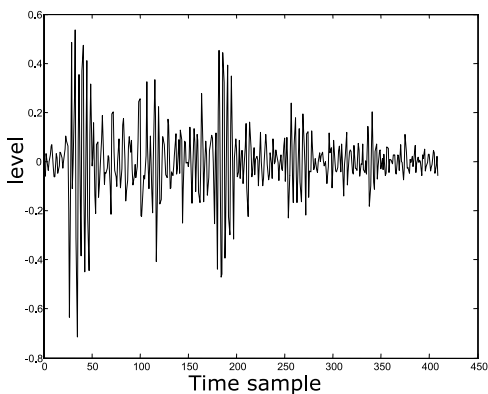
Fig. 13 Isolated click on right hydrophone
