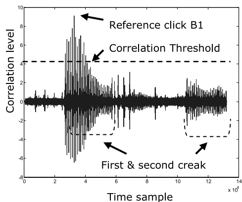
Fig. 7 Correlation with click B1
