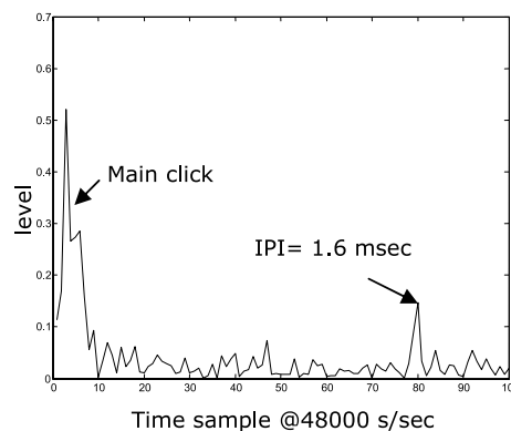
Fig. 10 Cepstrum of non-creak click A1
