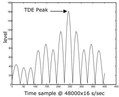
Fig. 14 Expanded view of auto-correlation peak of left hydrophone
