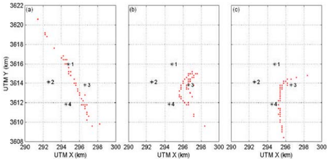
Figure 16. Point locations of the call tracks around the array with seismometer positions (1-4) indicated. Axes are for UTM Zone 11. Points indicate location estimates from many consecutive time windows, allowing tracking of a whale's path. Data are from the following time windows: (a) 08/28/01 02:52-04:52 (b) 08/28/01 09:33-13:50 (c) 08/29/01 02:55-04:50.
