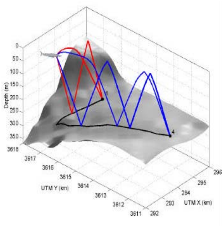
Figure 14. Predicted acoustic ray paths between a hypothesized whale and seismometers #1 and #4. Whale not drawn to scale. The range - dependent acoustic model allows for both direct and reflected ray paths to be included in the travel time calculation.
