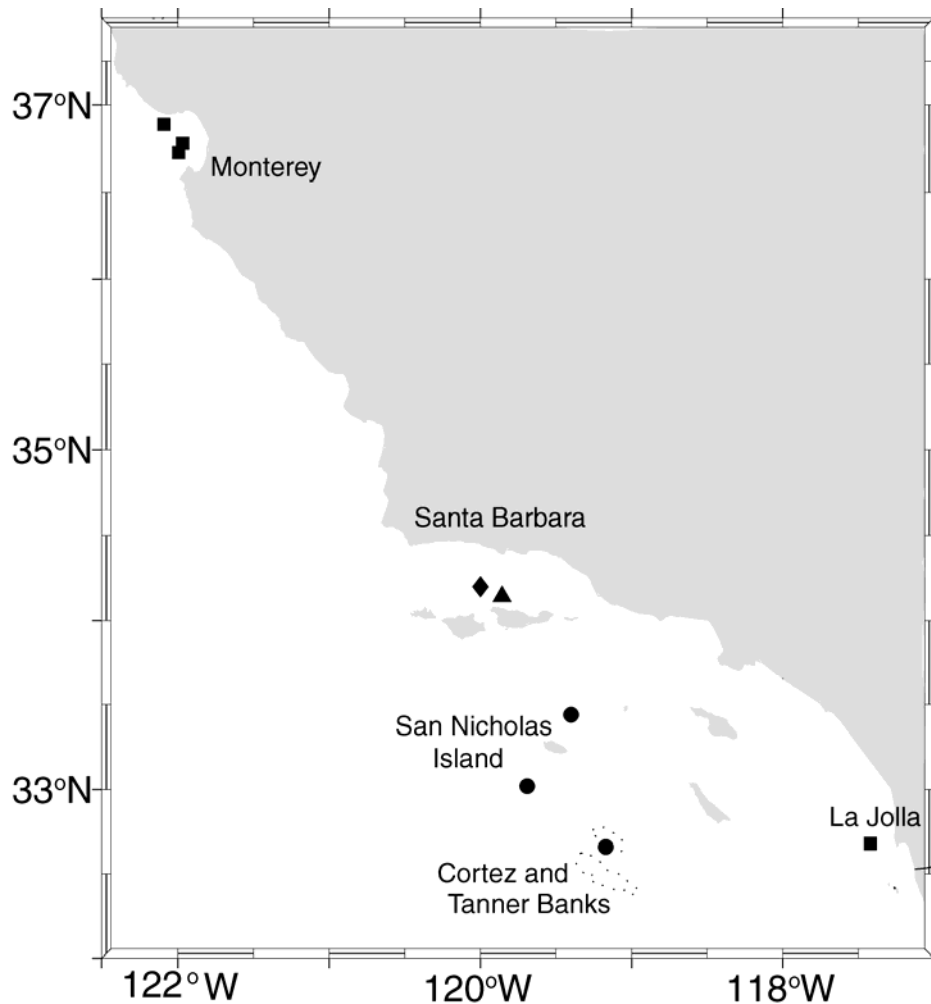
Figure 3. Blue whale study area in central and southern California. Symbols indicate the position of a tag deployment which recorded calls (■ = BProbe, ♦ = Crittercam, and ▲ = DTag), or the location of a skin sample of a calling whale.
