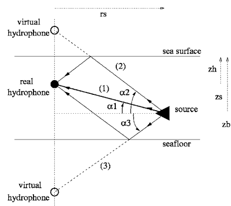
FIG. 2. Multipath ray geometry. The depths of the sperm whale, the hydrophone, and the seafloor are respectively z_s , z_h , and z_b . The sperm whale is at the range r_s from the hydrophone. The direct path ray, surface reflected ray, and seafloor reflected ray form the algebraic angles \alpha_1 ( \alpha_1 > 0 \Leftrightarrow z_s > z_h ), \alpha_2 ( \alpha_2 > 0 ), and \alpha_3 ( \alpha_3 < 0 ) to the horizontal. The detection of two surface/seafloor echoes serves as a substitute of a large virtual vertical hydrophone array of length 2z_b . The whale depth and range define the geometry of the multipath rays (length and inclination).
