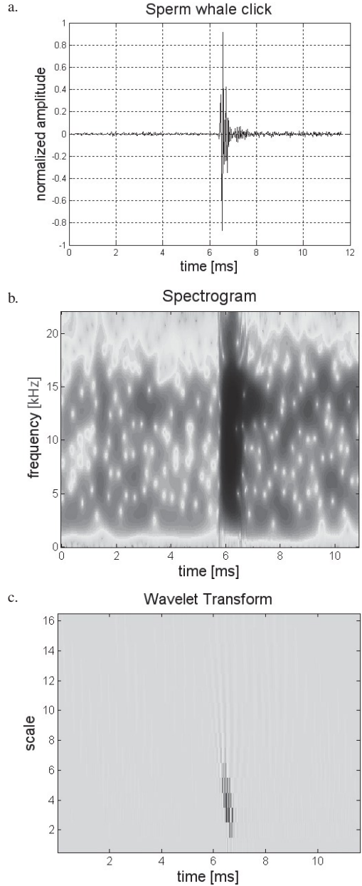
Figure 1. (a) Waveform of a typical sperm whale click; (b) spectrogram of this click; and (c) wavelet transform of this click
