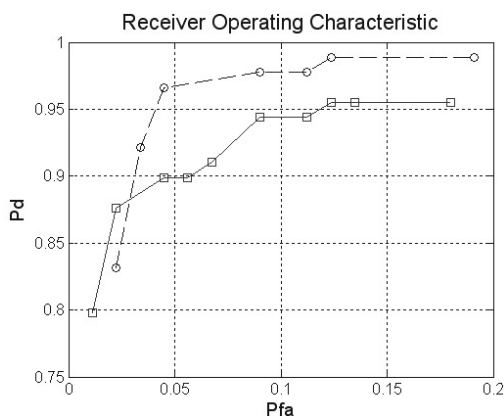
Figure 3. ROC curve of the two detectors ( STWE_{WT} - circles and STWE_{STFT} - squares)
