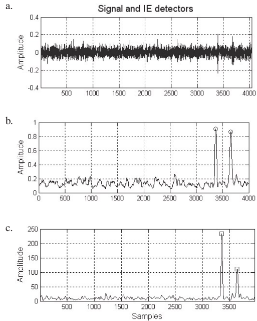
Figure 2. (a) Recorded signal with additional gaussian white noise (SNR = -10dB), containing two clicks; (b) detection with STWE_{WT} ; and (c) detection with STWE_{STFT}
