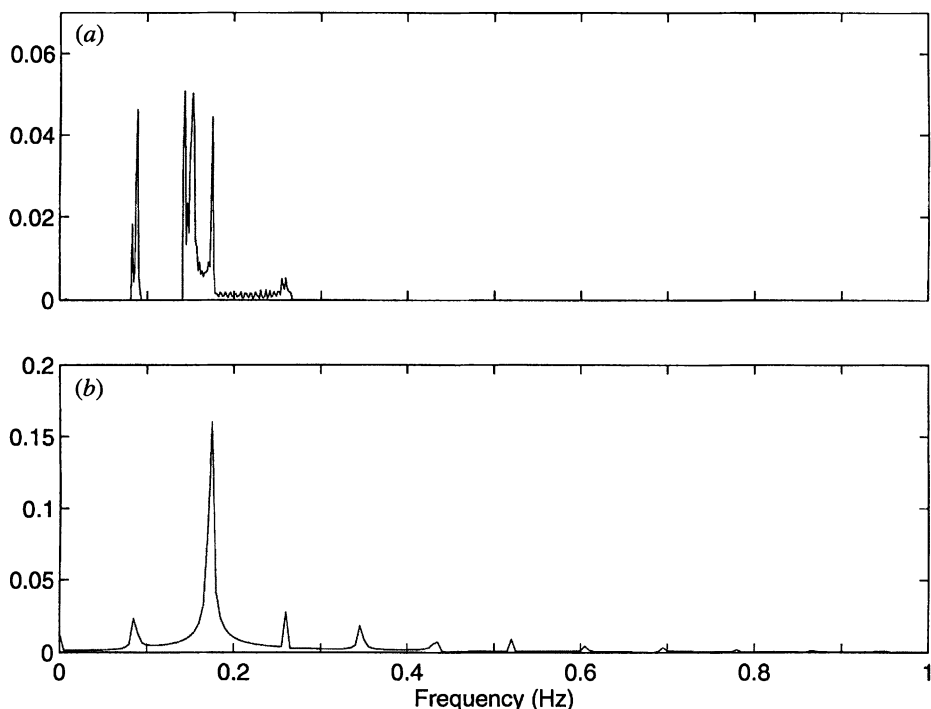
Figure 48. Comparison between the marginal spectrum and the Fourier spectrum for the Rössler equation: (a) the marginal spectrum showing the low-frequency oscillation near 0.1 Hz, and the high bimodal frequency distribution around 0.2 Hz generated by the intrawave frequency modulation; (b) the Fourier spectrum contains only harmonics with no indication of the two time scales involved in the period doubling. The main peak is the weighted mean of the physical time scales.
