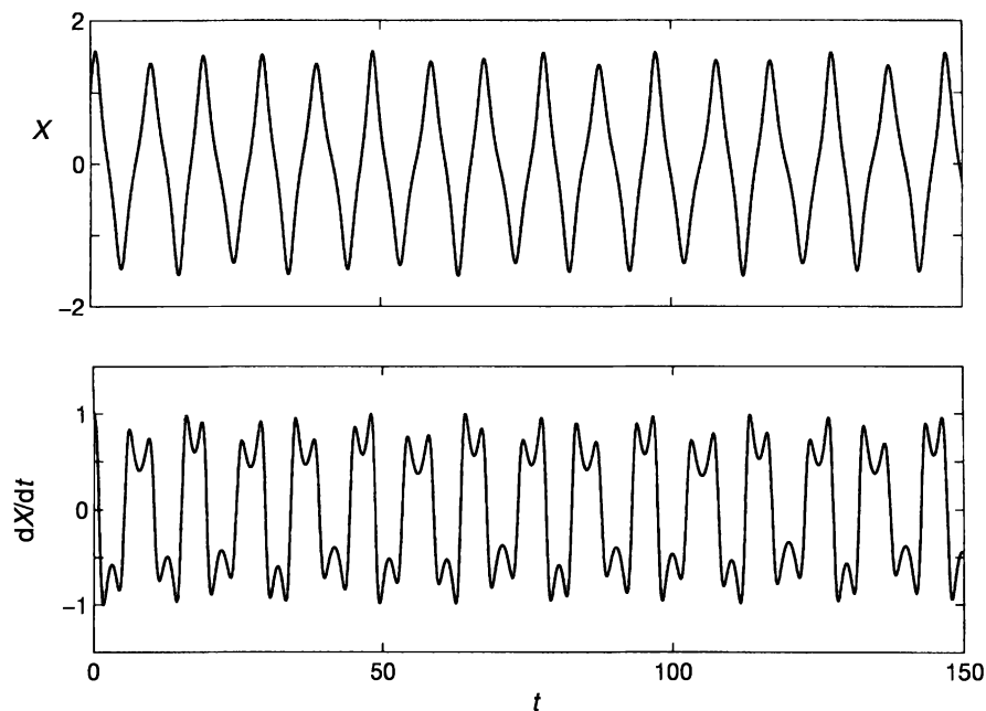
Figure 30. Numerical solution for the Duffing equation. The oscillation is highly nonlinear as indicated by the deformed wave-profile with pointed crests and troughs.
