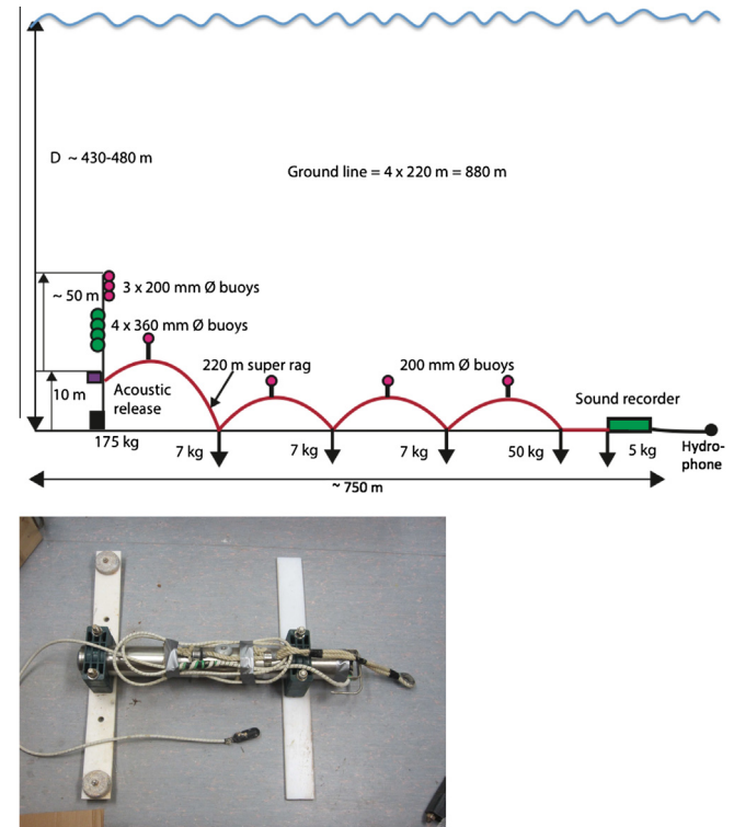
Fig. 2. Sketch of the IMOS passive acoustic mooring in the Perth Canyon (top panel) and photo of one CMST sound recorder (bottom panel).
