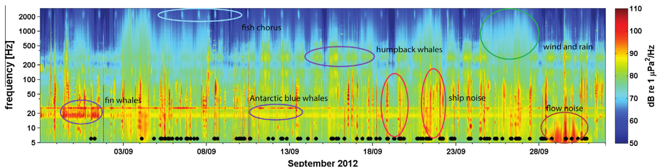
Fig. 3. Spectrogram for September 2012 showing the main contributors to the marine soundscape in the Perth Canyon. The black dots indicate ship passes within 20 km of the sound recorder (NFFT = 6000, fs = 6 kHz, 0% overlap).
