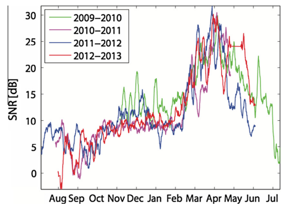
Fig. 14. Output of the pygmy blue whale detector from November 2009 to June 2013, demonstrating the presence of pygmy blue whales from November to June, peaking from March to June.
