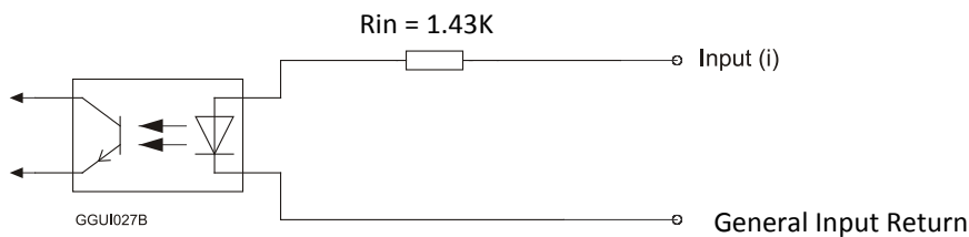
Figure 27: Digital Input Schematic
