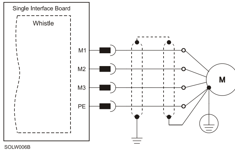
Figure 3: AC Motor Power Connection Diagram
