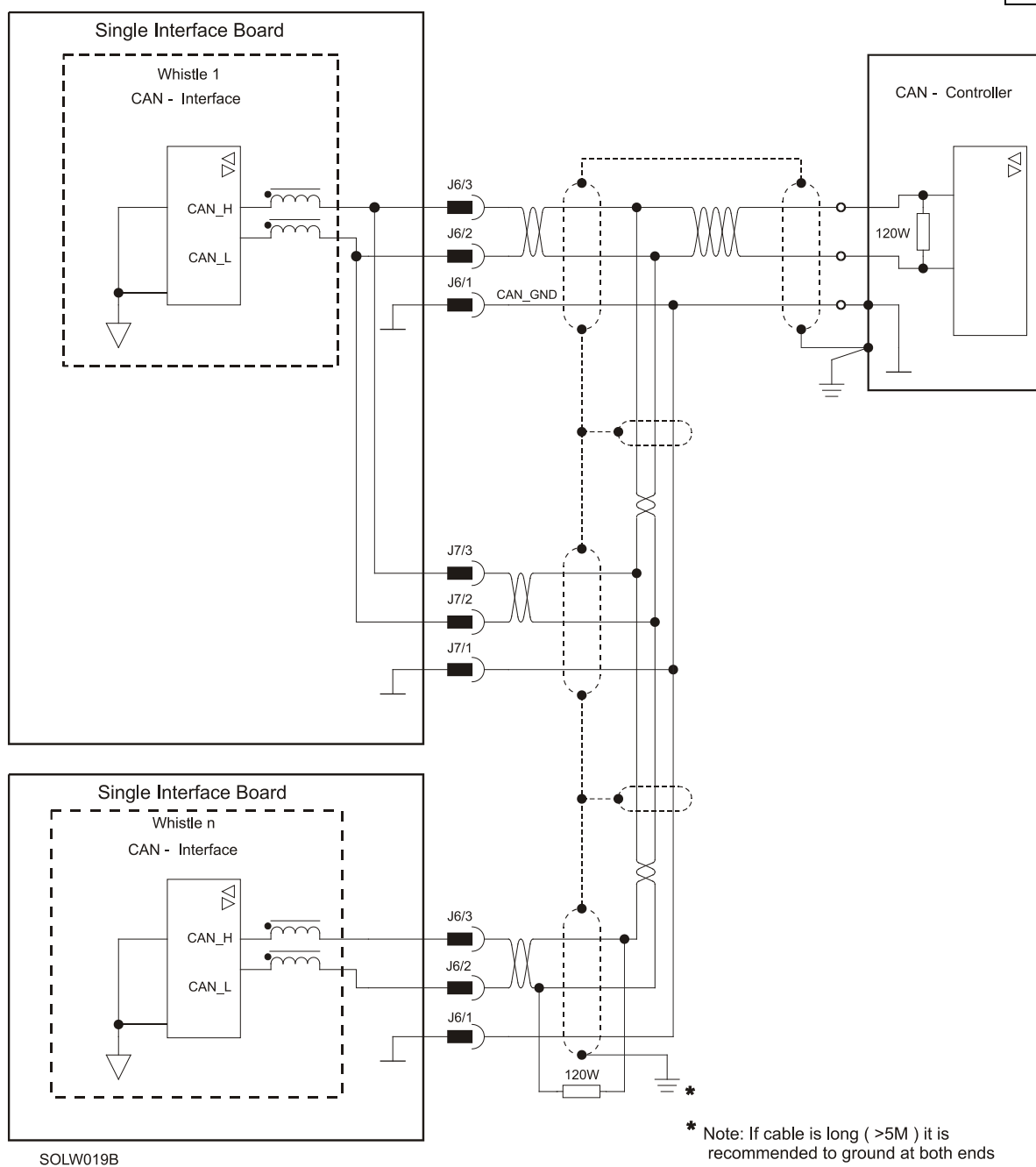
Figure 23: CANopen Network Diagram
