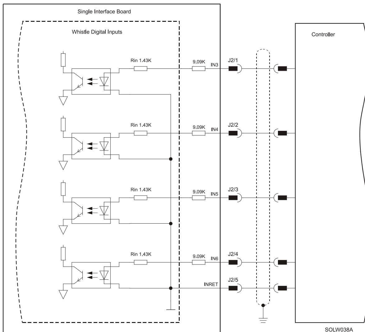
Figure 19: Digital Input 24 Connection Diagram
