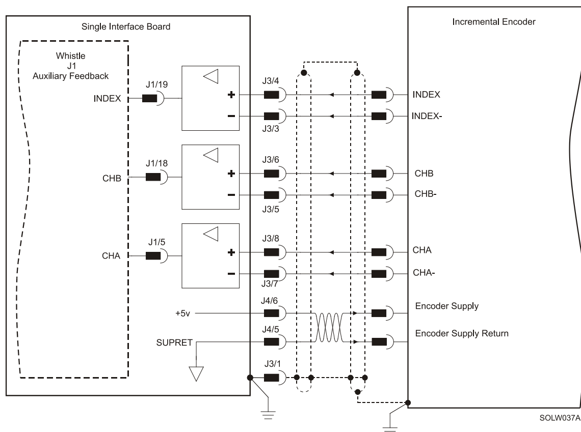
Figure 16: Differential Auxiliary Encoder Input Option Diagram
