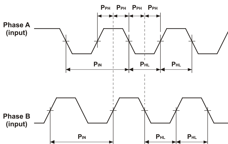
Figure 24: Main Feedback - Encoder Phase Diagram
