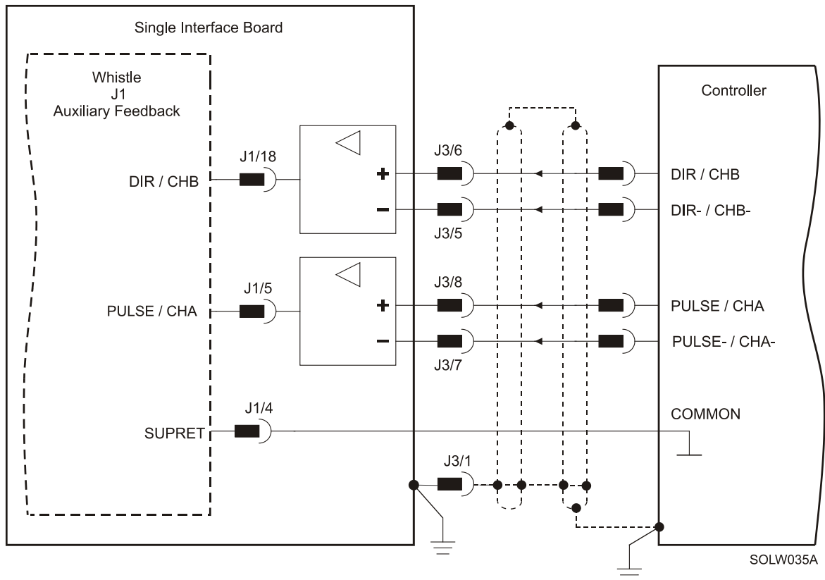
Figure 17: Pulse-and-Direction Diagram
