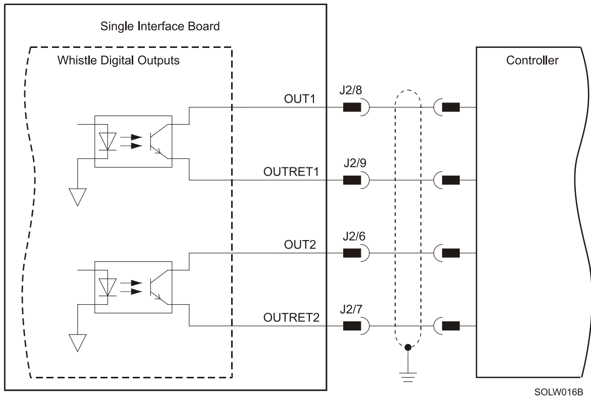
Figure 20: Digital Output Connection Diagram
