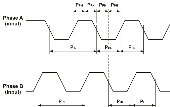
Figure 26: Auxiliary Feedback - Encoder Phase Diagram
