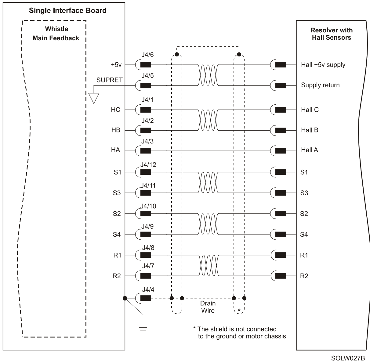
Figure 9: Main Feedback – Resolver with Digital Hall Sensor Connection Diagram
