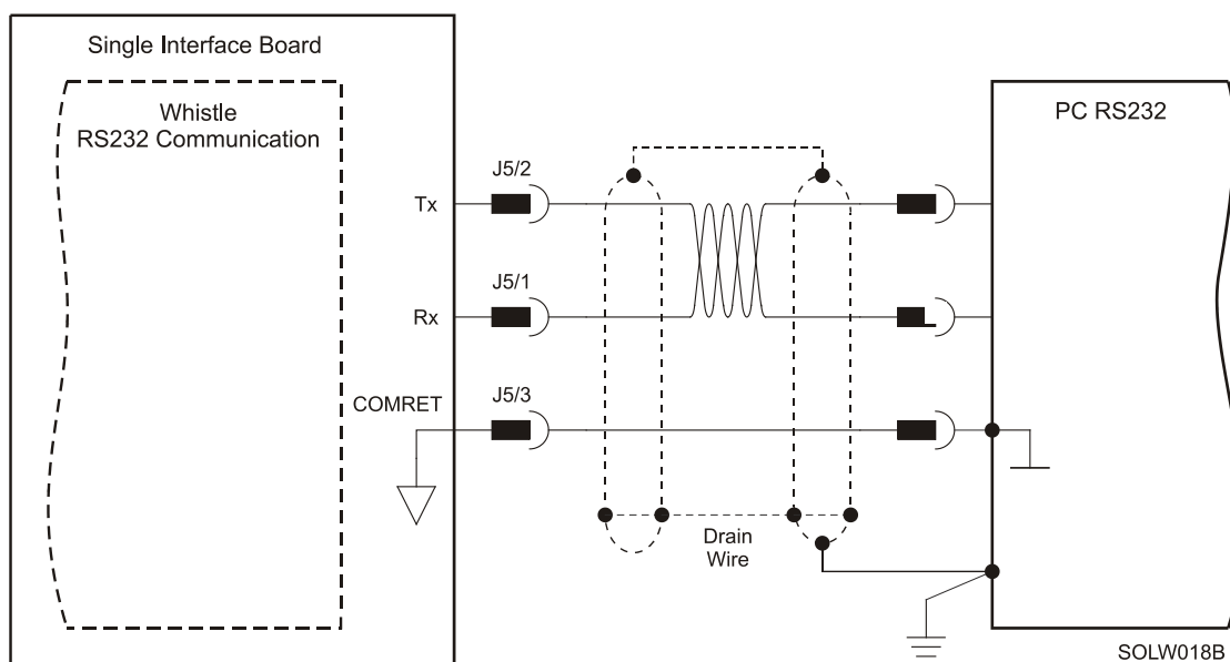
Figure 22: RS-232 Connection Diagram
