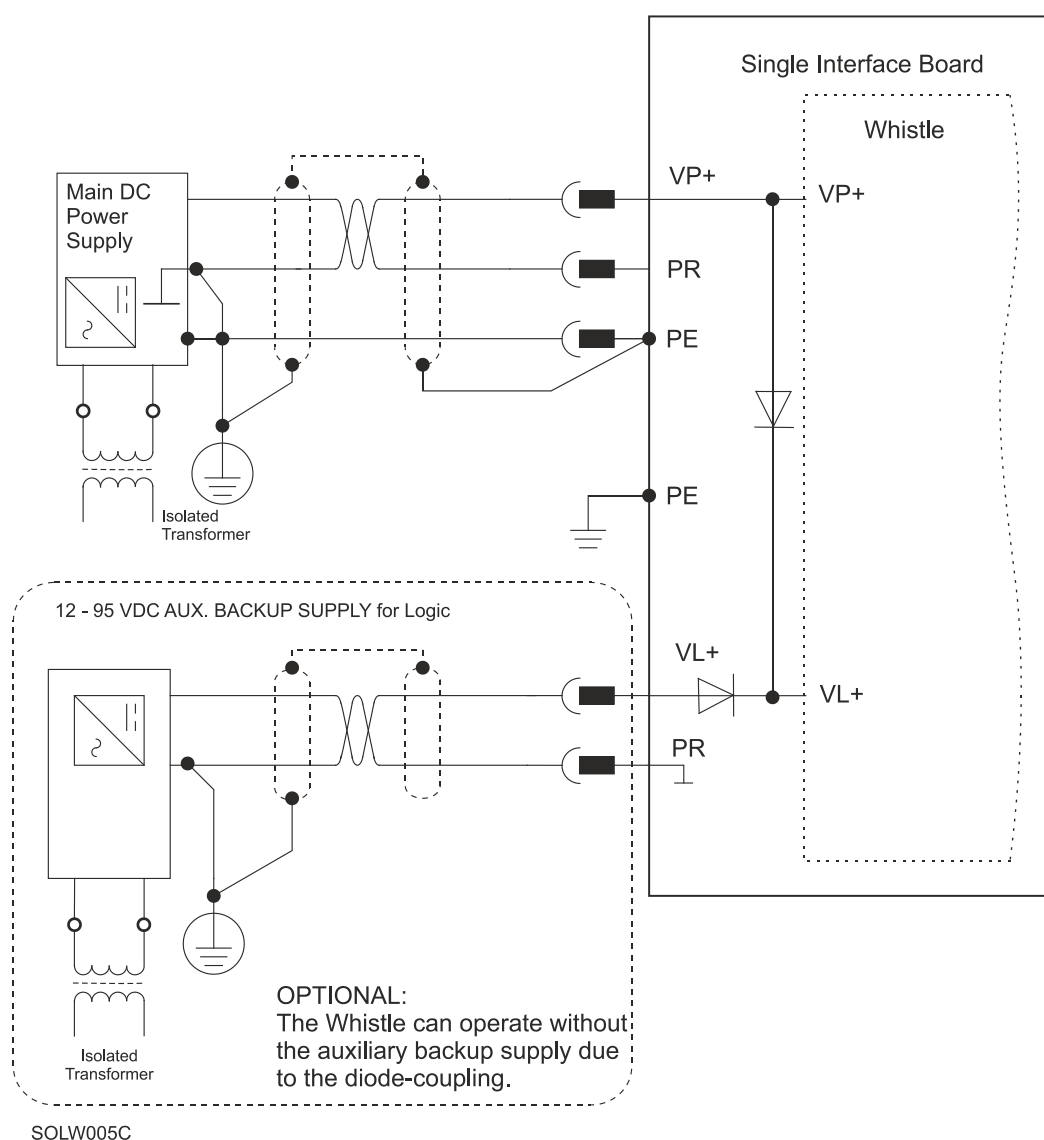
Figure 4: Main Power Supply Connection Diagram
