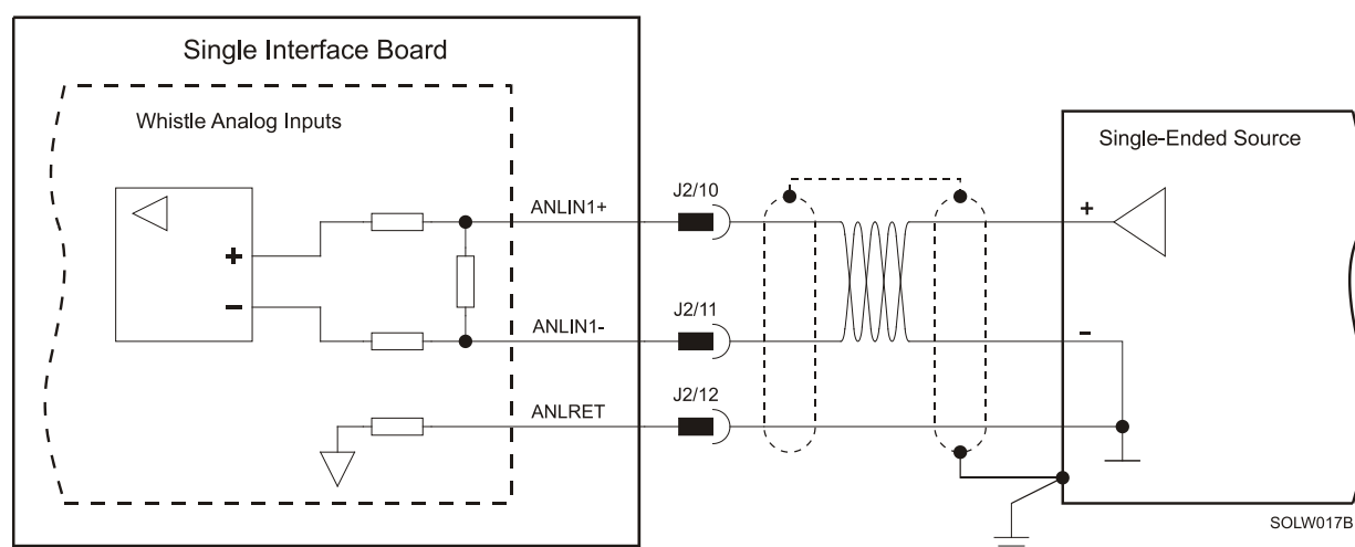
Figure 21: Analog Input with Single-Ended Source
