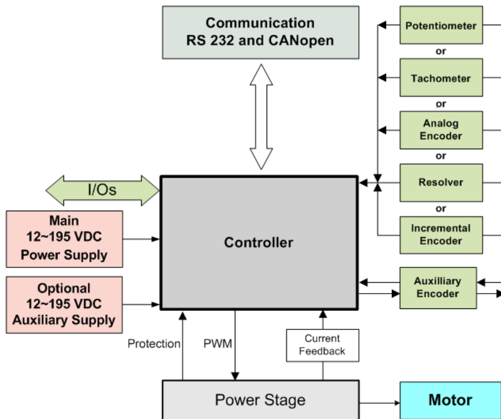
Figure 1: Solo Whistle System Block Diagram
