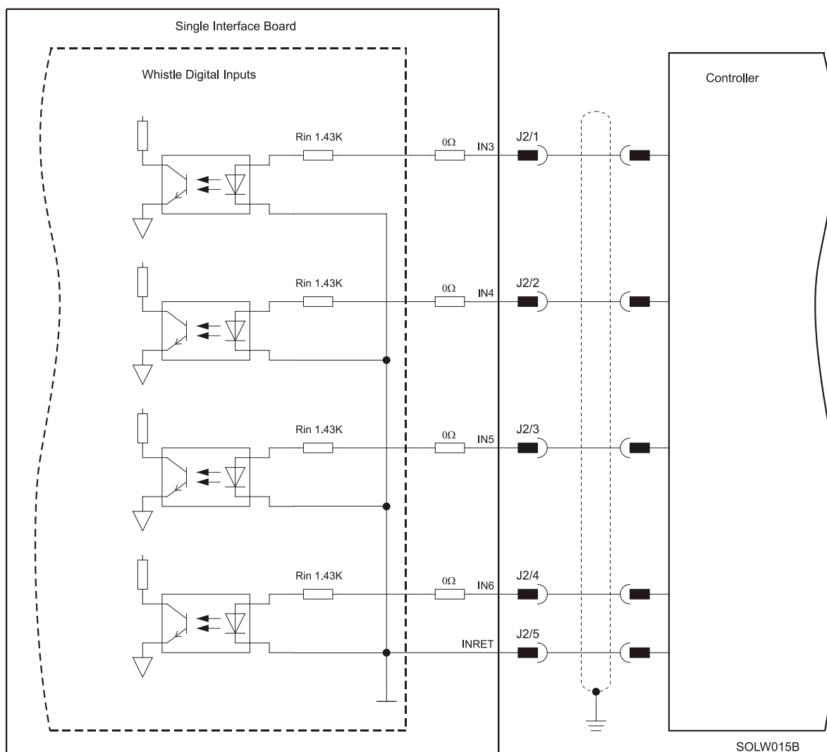
Figure 18: Digital Input 5 V Connection Diagram
