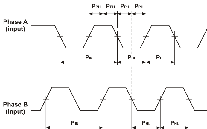
Figure 25: Auxiliary Feedback - Encoder Phase Diagram
