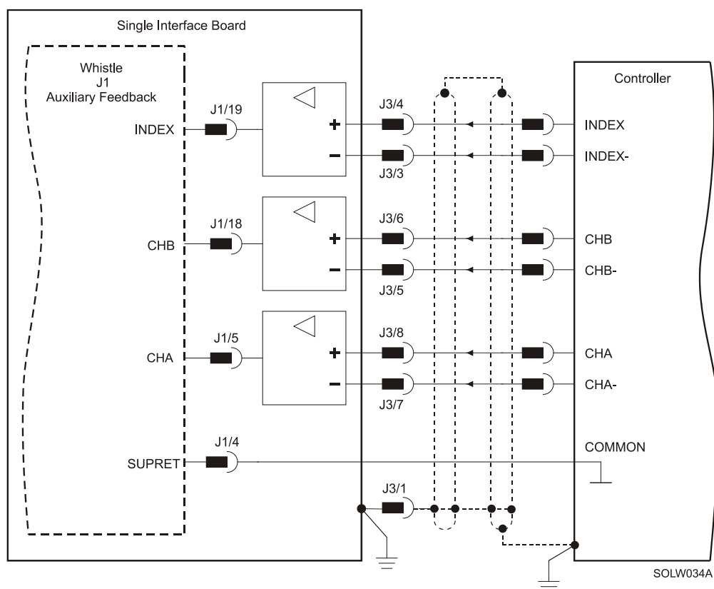
Figure 15: Differential Auxiliary Encoder Input Option Diagram
