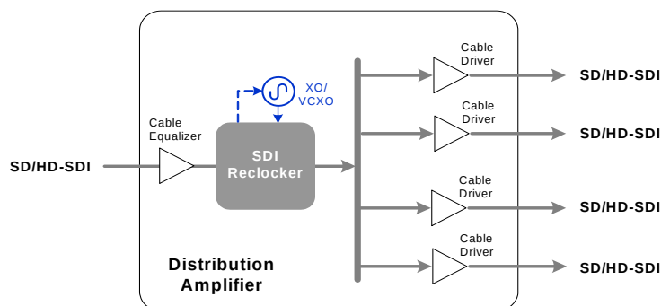
Figure 6. Block Diagram of a Distribution Amplifier
