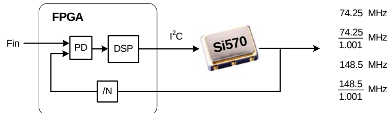
Figure 17. FPGA-Based DCXO PLL Supporting Multiple Video Standards
