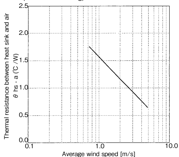
Figure 2-8 Thermal resistance cahracteristic in relation to wind speed for the heat sink prepared for [HAH-15L]
