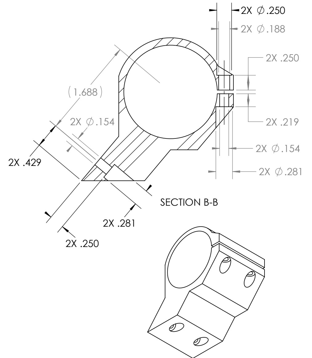
R.P. in ABS mat'l, COLOR: NATURAL FORTUS 400 - TIP SIZE .005
