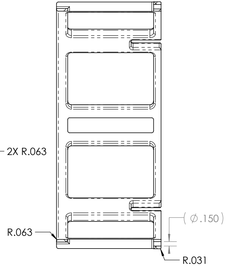
SECTION C-C
