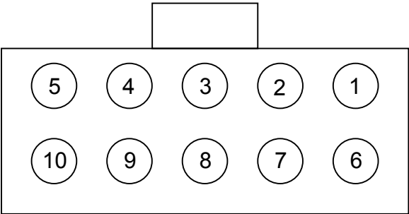
794196-1 FACE VIEW
