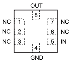
Pin Functions
