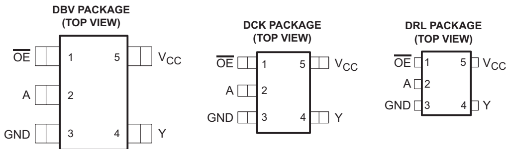
Pin Functions
