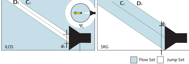
Fig. 4. Representation of the sets C_1, C_2, D_1, D_2 for the hybrid guidance that dictates the switches among ILOS and SRG.
