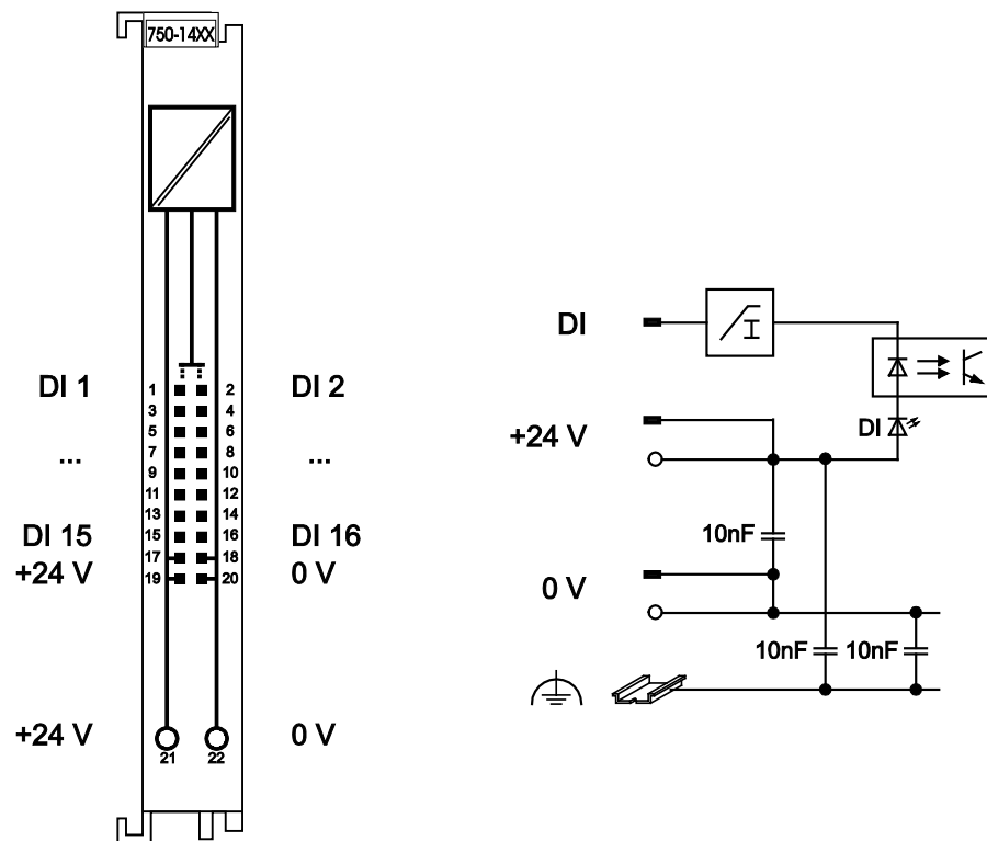
Figure 5: Schematic Diagram
