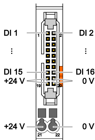
Figure 3: Connectors
