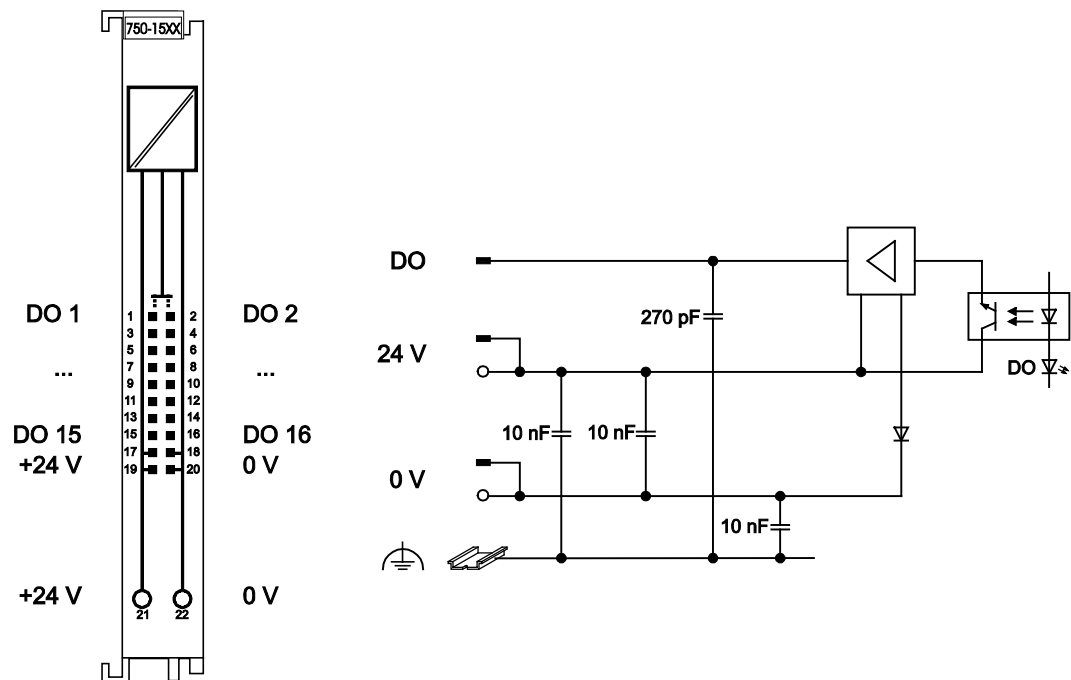
Figure 5: Schematic Diagram
