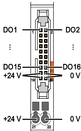
Figure 3: Connectors
