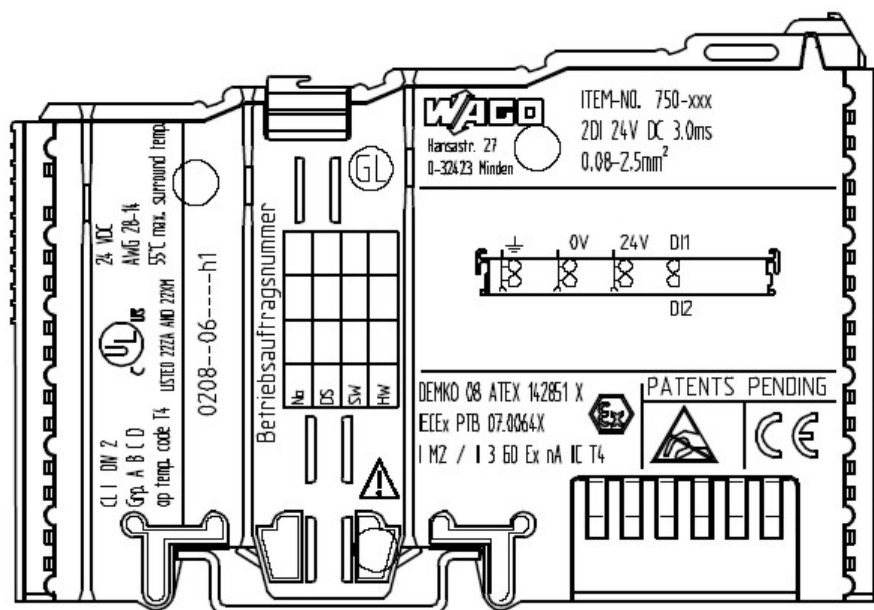
Figure 13: Side marking example for ATEX and IEC Ex approved I/O modules according to CENELEC and IEC
