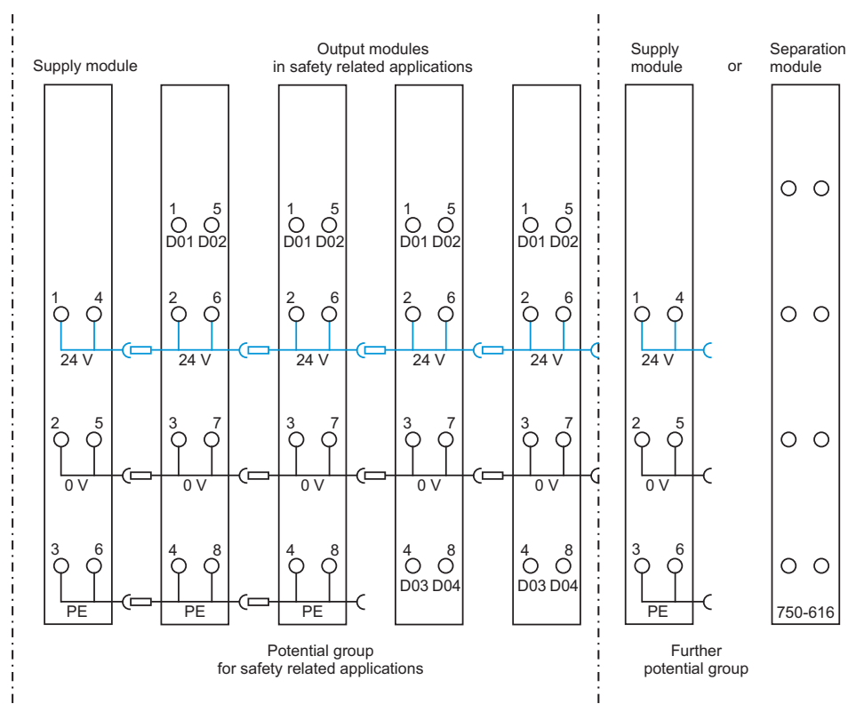
Figure 10: Potential group for safety related applications
