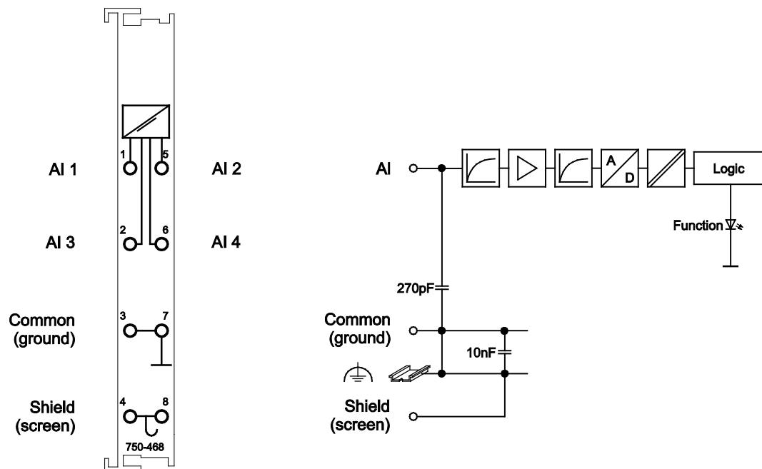
Figure 5: Schematic Diagram
